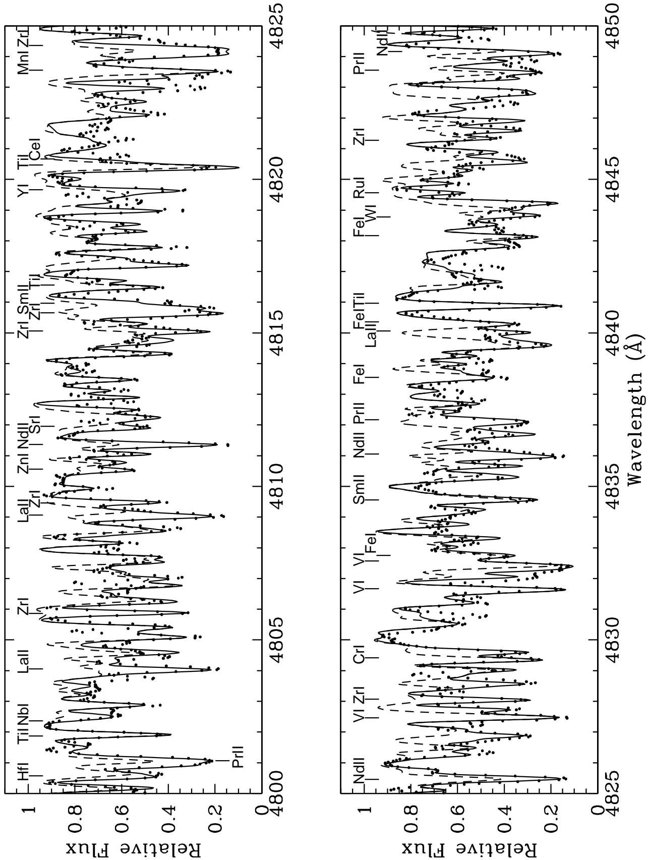
Fig. 2. Synthetic fits to the spectrum of the star IGI95-C1 in the region around 4825 Å. From this region we derived most of the s-elements abundances and the mean metallicity of the stars. Some atomic lines, main contributors to the specific spectral feature, are marked. Black dots represent the observed spectrum. Lines are synthetic spectra: only molecules and metals (dashed line), and including s-elements (best fit, continuous line).
