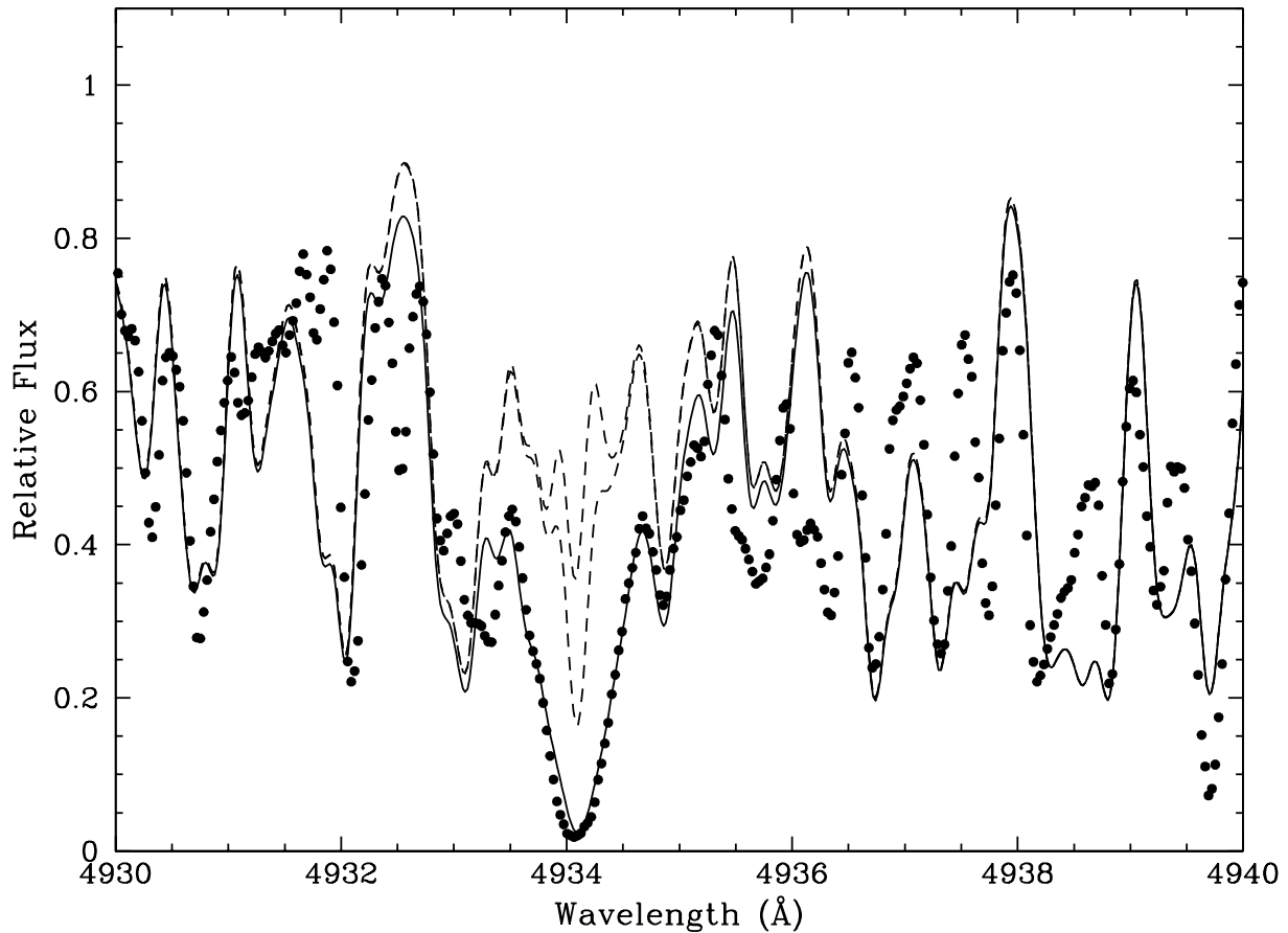
Fig. 3. Synthetic fit to the spectrum of IGI95-C1 in the region of the Ba II line at \lambda 4934 \text{ \AA} . Black dots are the observed spectrum. Lines are synthetic spectra for different [Ba/M] ratios: no Ba and +0.0 (dashed lines), +1.5 (best fit, continuous line).
