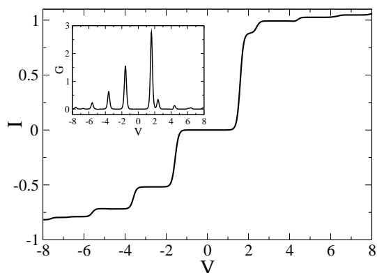
FIG. 17: Asymmetry of I(V) due to "half-shuttle": s = 0.1 (solid) and s = 0 (dashed). The case of \alpha = 0.7 , c_l = 0.75 , E = 0 , T = 0.04 . The inset shows the differential conductance for s = 0.1 .
