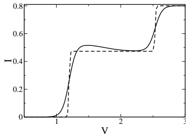
FIG. 13: The NDC induced by temperature for the case \alpha = 0.8 , c_l = 0.25 , E = 0.9 : T = 0.005 (dashed) and 0.04 (solid).
