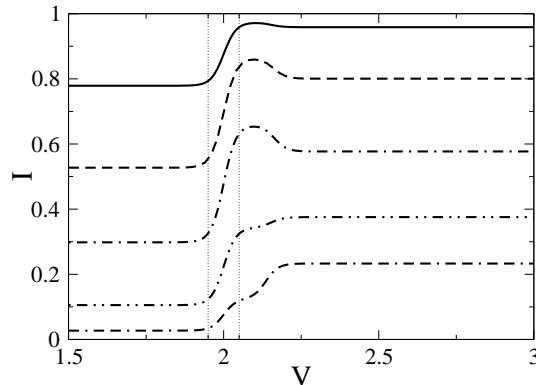
FIG. 8: From up to down \alpha = \{0.5, 0.8, 1.1, 1.5, 1.9\} for c_l = 0.5 . T = 0.01 . The dotted vertical lines around V = 2 (corresponding to V_{\pm} = 2 \pm 0.05 ) show the width of the Fermi distribution function at given T .
