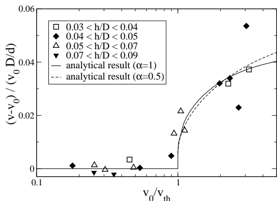
FIG. 7: Large bubble relative velocity in rescaled units (same data as in Fig. 6). The mean flow velocity threshold v_{th}(D) used to rescale the experimental data, is obtained from eq.7. The first analytical result (full line) is obtained from eq. 6, with the adjustable prefactor 0.045. Numerical simulations in vertex model have been performed, leading to a good agreement with theory as well, with an adjustable prefactor of 0.07 [9]. The second curve (dashed line) is the exact solution of eq. 5, using the experimental value of \alpha ( \alpha = 0.5 ), with an adjustable prefactor (see [9]).
