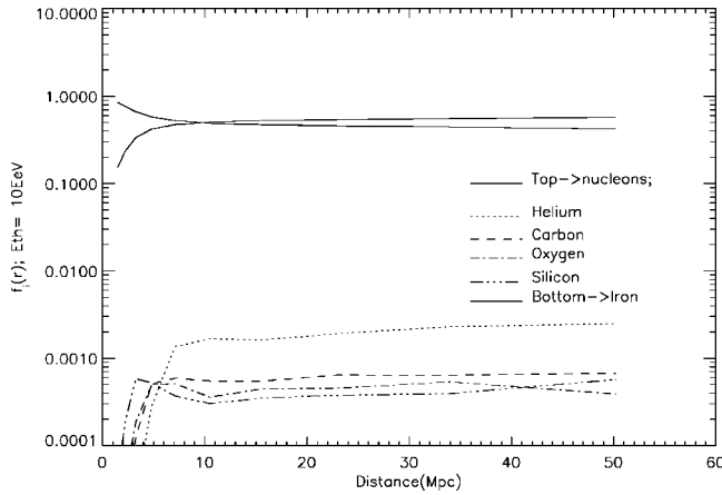
FIG. 4. Relative chemical composition above 10^{19} eV as a function of the distance for B = 10^{-12} G.
