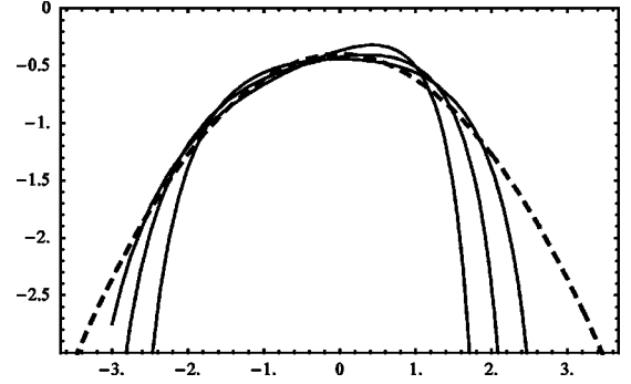
FIG. 2. PDF of \delta\chi_S = \delta\chi_S - \bar{\chi} for different values of \bar{\chi} . The dashed line corresponds to a Gaussian distribution; the dot-dashed line to the deformed distribution of \delta\chi_S when \lambda N_e/H^2=1 and \bar{\chi}=0 , and the solid lines to the deformed distribution when \bar{\chi} equals 0.5 and 1.
