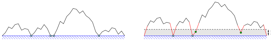
Figure 10: The transformation: A random subset of the pinned sites is unpinned and the height at the corresponding sites is chosen at random in the interval (0, 1) . To avoid overcounting, the whole interface, except the pinned sites, is lifted by 1 before this procedure is applied.
