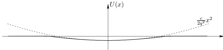
Figure 8: The pinning potential considered in [46] and its quadratic approximation yielding the effective mass.
