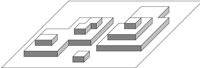
Figure 4: A picture of the wedding cake model. Gradients can take only values 0 and \pm 1 , and the interface height can only increase. The level lines of this model are exactly identical to the contours of the Ising model.
