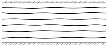
Figure 6: A stack of interfaces between two fixed walls. Another variant consist in an infinite “one-dimensional” gas of d -dimensional interfaces with positive fugacity.
