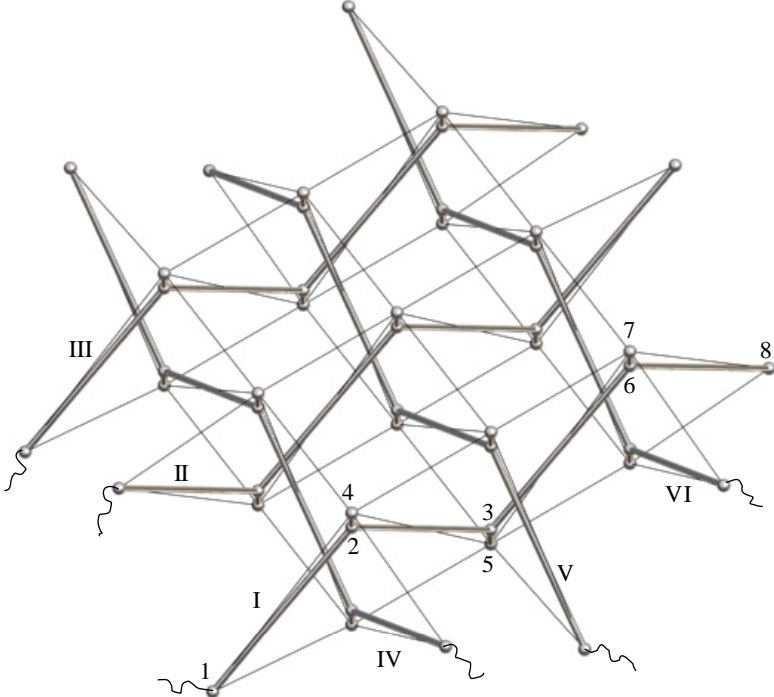
Figure 11. Self-stress truss member assembly (bidirectional grid)
