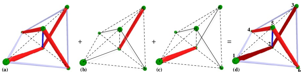
Figure 5. Various states of self-stress in module 2V taken from the computer simulation generated by the T2000 program, (a) global self-stress, (b,c) local self-stress, (d) total self-stress
