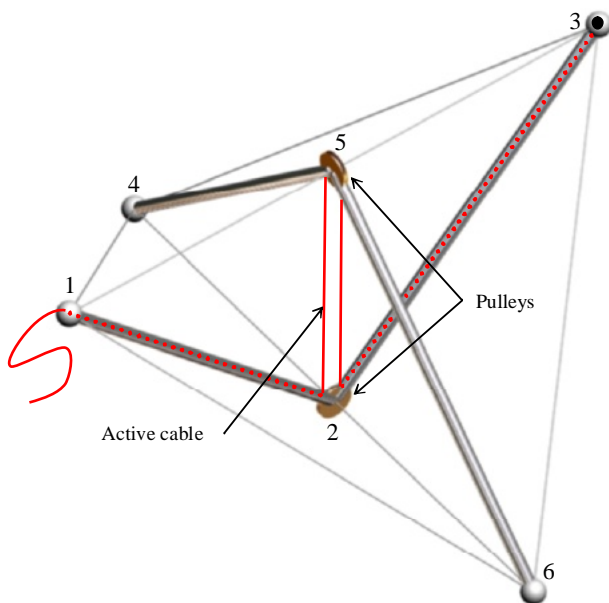
Figure 3. Cable path (1-2-5-2-3)
