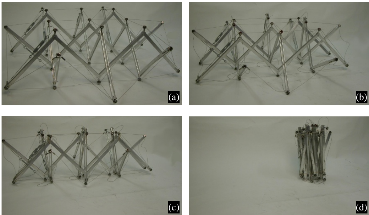
Figure 13. Folding of the grid, physical model
