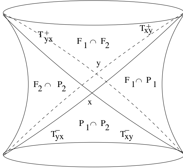
FIGURE 3. The splitting case. The domain E(\Lambda) is between the hyperplanes x^\perp and y^\perp . These hyperplanes, tangent to the hyperboloid, are not drawn, except their intersections with the hyperboloid, which are the upper and lower tents \mathcal{T}_{xy}^\pm, \mathcal{T}_{yx}^\pm .
