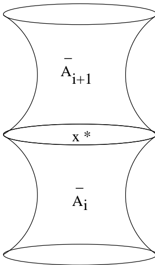
FIGURE 1. Universal anti-de Sitter space as a sum of affine domains.
