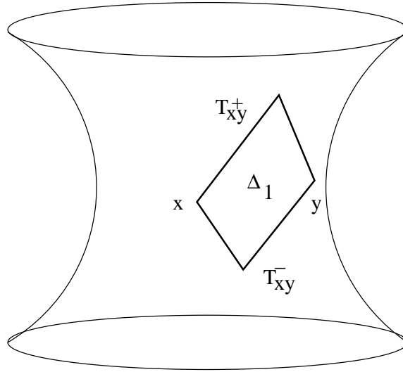
FIGURE 2. Upper and lower tents
