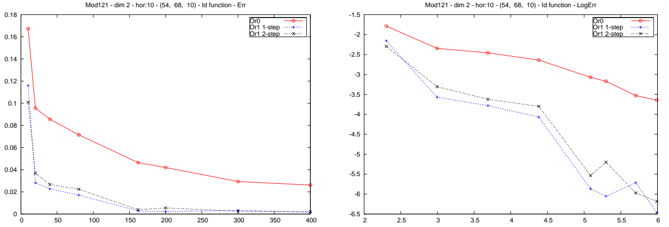
Figure 5: Quantization filter estimator errors for 2-dimensional Kalman case as a function of the quantizer size N_k (left: \|\Pi_{10} f_1 - \hat{\Pi}_{10} f_1\|_2 , right: log-log scale representation).
