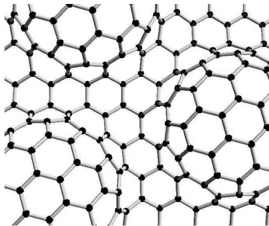
FIG. 5: Embryos of (12,0) SWNTs, seen from above, arranged in an hexagonal network. In this case, the growth is possible without creation of dislocations (see text).
