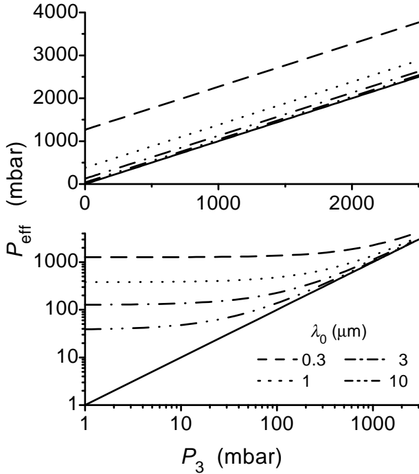
FIG. 11: Broken lines: Pressure dependence of P_{\text{eff}} = \mathcal{D}_3/D_{\text{eff}} [Eq. (S-2), with f(\lambda) \propto \exp[-(\lambda - \lambda_0)^2/\delta\lambda^2] ], computed for various mean values \lambda_0 (see legend) and \delta\lambda = 0.01 \mu\text{m} . Solid line: free gas data ( P_{\text{eff}} = P_3 ).
