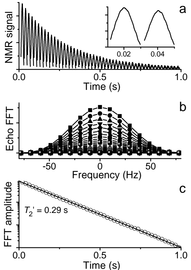
FIG. 4: a: Example of spin-echo train obtained in aerogel A (with 33.4 mbars of ^3\text{He} plus 616.5 mbars of \text{N}_2 , G = 0.314 mT/m, and T_{CP} = 21 ms). Saturation of the detection system by the strong rf pulses occurs between echoes (data points removed). Inset: Blow-up plot of first and second echoes. b: Fast Fourier transforms (FFTs) of the consecutive echo data sets, identified by individual symbol shapes. c: Exponential fit of FFT decay, yielding T_2' = 0.29 s.
