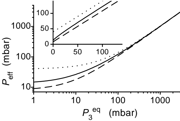
FIG. 13: Pressure dependence of P_{\text{eff}} obtained for a bimodal mfp distribution (solid line) that combines two narrow Gaussian distributions : \lambda_0 = 50 \mu\text{m} , \delta\lambda = 0.1 \mu\text{m} (distribution f^{(1)} , dashed line), and \lambda_0 = 10 \mu\text{m} , \delta\lambda = 0.1 \mu\text{m} (dotted line), in log plot. Inset: linear plot, for the same distributions.
