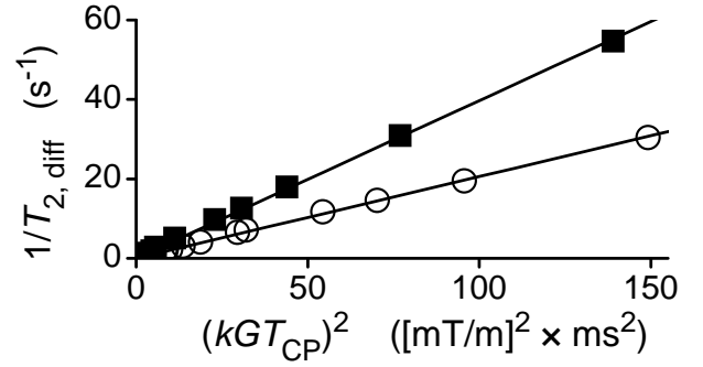
FIG. 6: Compilation of spin-echo decay rates measured in the reference cell (solid squares) and in aerogel M (open circles) at fixed gas pressures. Diffusion-weighting parameter (kGT_{CP})^2 is varied through changes of gradient strengths ( G : 0.07–2.2 mT/m) and echo times ( T_{CP} : 4.4–31 ms). The expected linear dependence [Eq. (2)], observed over more than two decades, yields D_{\text{gas}} = 1.148 \pm 0.004 cm 2 /s in the reference cell, and D_{\text{eff}} = 0.595 \pm 0.008 cm 2 /s in aerogel M, for the two ^3\text{He} - \text{N}_2 mixtures used ( P_3^{\text{eq}} = 1.41 bar and 1.70 bar, respectively - see Section IV A).
