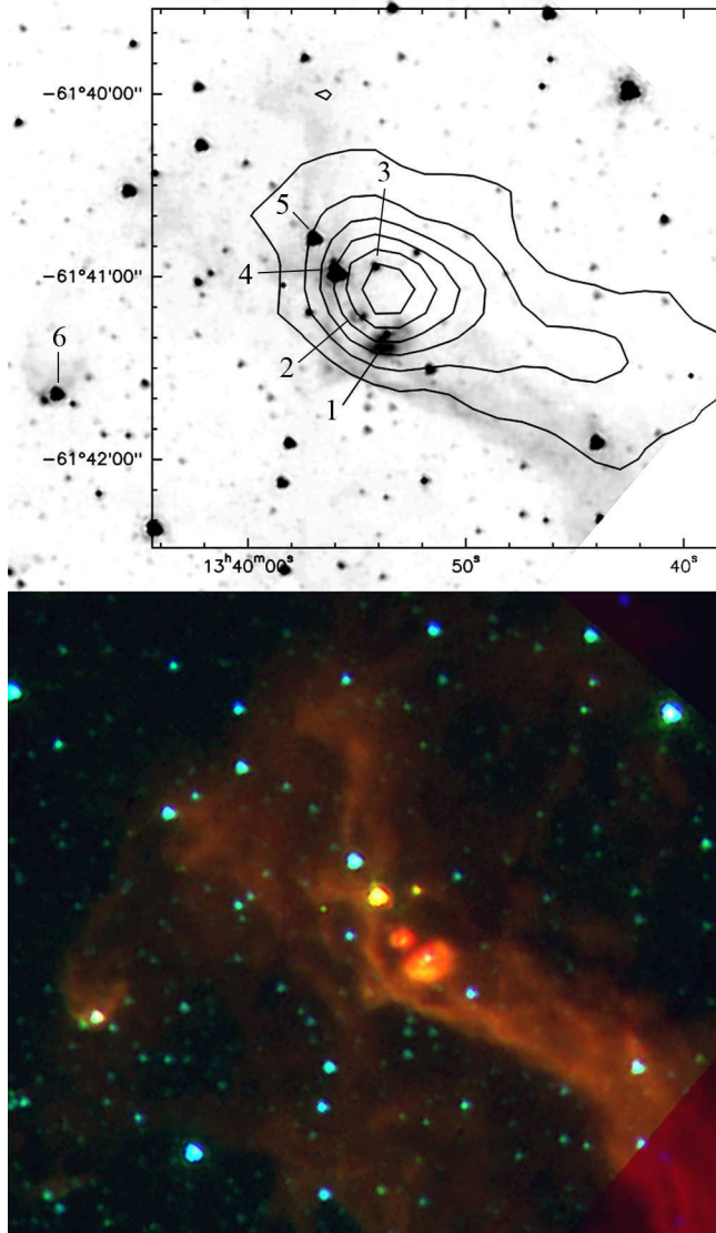
Fig. 6. As Fig. 4 but for condensation 4
