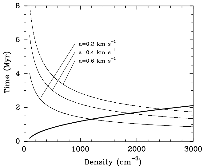
Fig. 13. Variations of t_{\text{dyn}} (thick curve) and t_{\text{frag}} (thin curves) as a function of the density, n_0 , for the observed radius of 6.4 pc and three values of a_s (0.2, 0.4, and 0.6 km s -1 ), respectively
