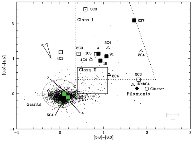
Fig. 9. GLIMPSE colour-colour diagram, [3.6]-[4.5] versus [5.8]-[8.0] , for the sources observed towards the most massive condensations detected at 1.2-mm (nos 2, 3 and 4) and the sources observed in the RCW 79 field (small black dots), extracted from the GLIMPSE PSC. The sources observed towards the compact H II region are identified by their numbers in Table 3 and shown as filled squares. The sources observed towards condensation 3 are shown as empty squares and identified by their numbers in Table 3 plus C3 (i.e. 1C3 for object 1 of condensation 3). Same for sources observed towards condensation 4, shown as empty triangles. The locations of Class I and II YSOs and red giants are from Allen et al. (2004) and Whitney et al. (2004). Extinction vectors are shown for A_V=30 mag, taken from Allen et al. (2004). The stars discussed in the text are identified. Typical error bars are shown
