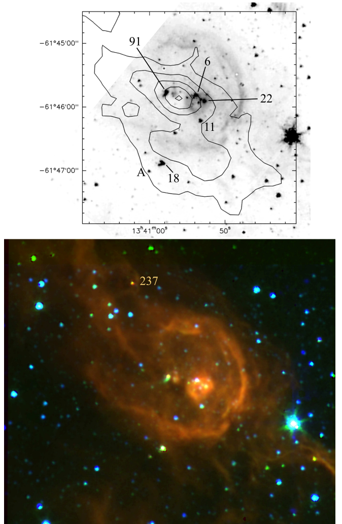
Fig. 4. Condensation 2 - Top) The 1.2-mm continuum emission is superimposed, in contours, on the 3.6 \mu\text{m} image taken from the Spitzer GLIMPSE survey. Bottom) Color composite image combining the K_S image from the 2MASS survey (in blue), and the 3.6 \mu\text{m} (in green) and the 8 \mu\text{m} (in red), both from the GLIMPSE survey. The stars discussed in the text are identified by their numbers in Table 3
