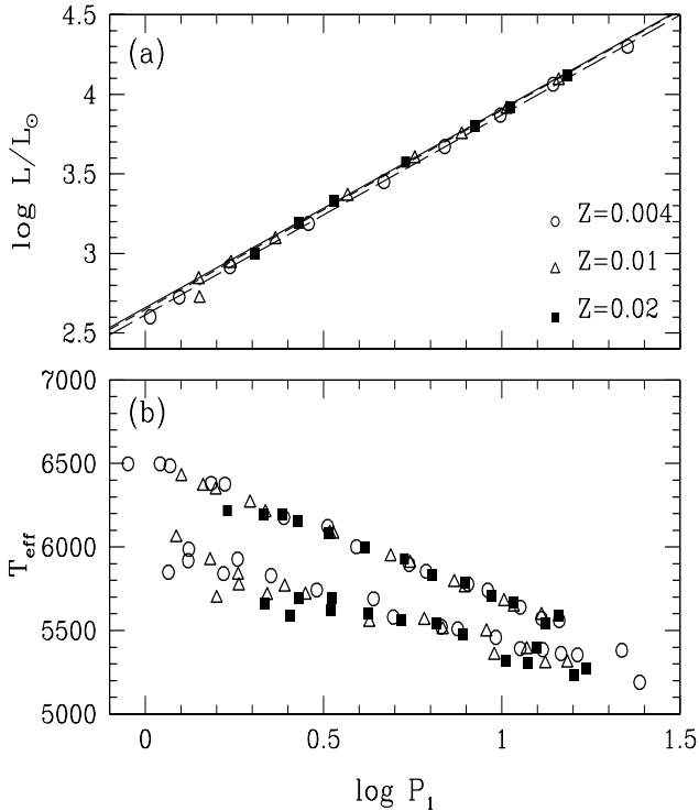
Fig. 1. a) \log P (in days) – L diagram for 1H pulsators and different metallicities. The symbols indicate the mean position of each mass in the IS as a function of Z . The mean PL relationships are plotted for Z = 0.02 (solid line), Z = 0.01 (dashed line) and Z = 0.004 (long dashed-line). b) Location of the blue and red edges of the 1H IS in a \log P - T_{\text{eff}} diagram. The symbols correspond to the same Z as in a) . The minimum masses undergoing a blue loop in the IS are 3.25 M_{\odot} , 4 M_{\odot} and 5 M_{\odot} for respectively Z = 0.004 , 0.01 and 0.02
