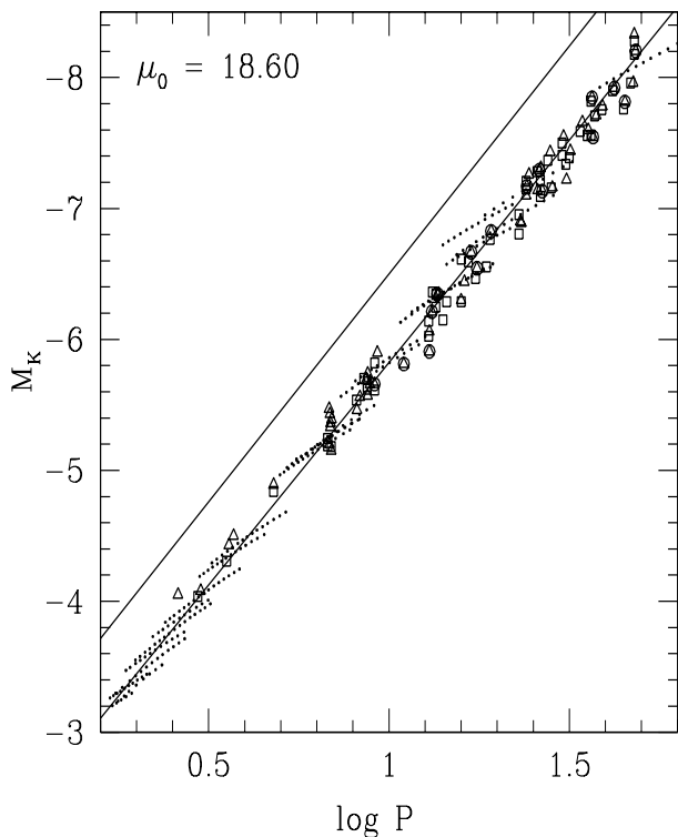
Fig. 6. \log P (in days) – M_K diagram for LMC observed Cepheids. The dots correspond to models for fundamental mode pulsators during core He burning, with Z = 0.01 . The open squares are from Persson et al. (2000). The triangles are observations from Gieren et al. (1998). The open circles are from Laney & Stobie (1994). The 2 solid curves are the theoretical mean PL relationships for respectively F (lower curve) and 1H (upper curve)
