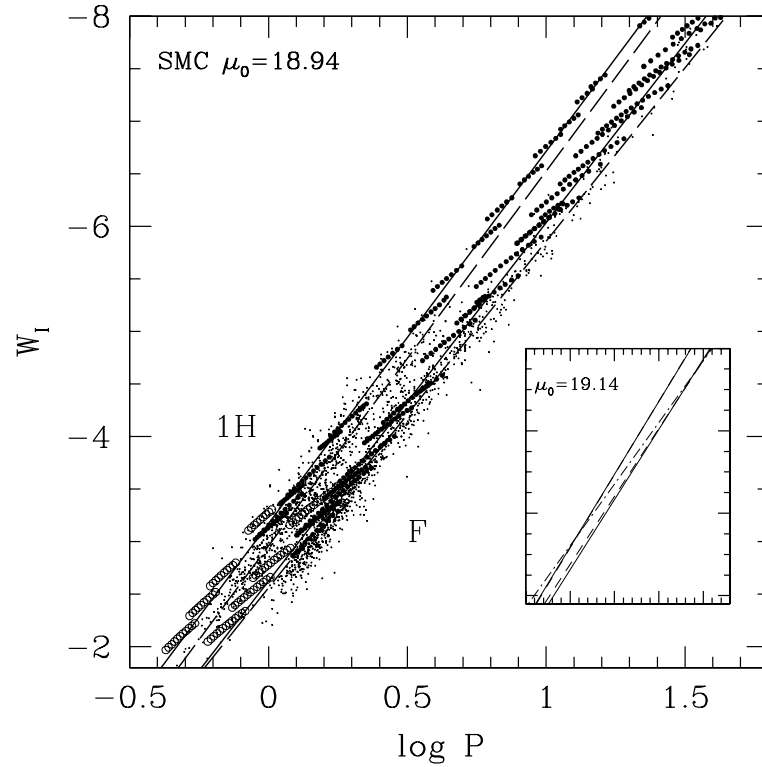
Fig. 4. \log P (in days) – W_I diagram for F and 1H pulsators for models with Z = 0.004 and SMC observed Cepheids. Symbols and curves are the same as in Fig. 2. The inset displays only the mean relationships with the same linestyle as in the main figure for a distance modulus \mu_0 = 19.14 . The dash-dotted curve corresponds to the F relationship of Caputo et al. (2000). Note that for 1H, the theoretical and observed mean relationships are indistinguishable in the inset
