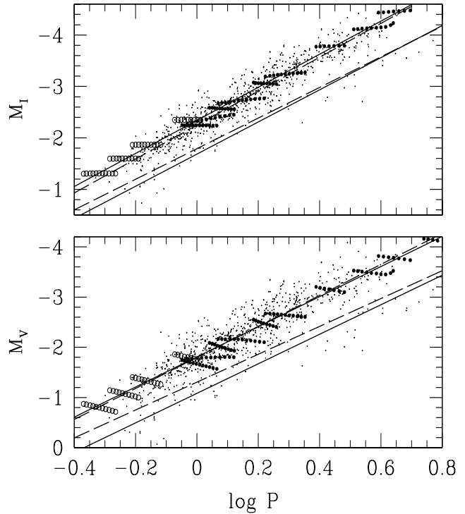
Fig. 2. Period (in days) – magnitude diagrams for 1H pulsators in the VI bands for models with Z = 0.004 and SMC observed Cepheids. The filled circles correspond to unstable 1H modes during core He burning phase from m_{\text{min}} = 3.25 M_{\odot} to 6 M_{\odot} . The large open circles correspond to first crossing unstable 1H modes for 3, 3.25, 3.5 and 4 M_{\odot} . Observations (dots) are from OGLE2 (Udalski et al. 1999b). The distance modulus is 18.94. The 2 solid curves are the theoretical mean PL relationships for respectively F (lower curve) and 1H (upper curve) pulsators. The long-dashed curves are the observed PL relationship derived by Udalski et al. (1999c) and Udalski (2000) for F and 1H pulsators
