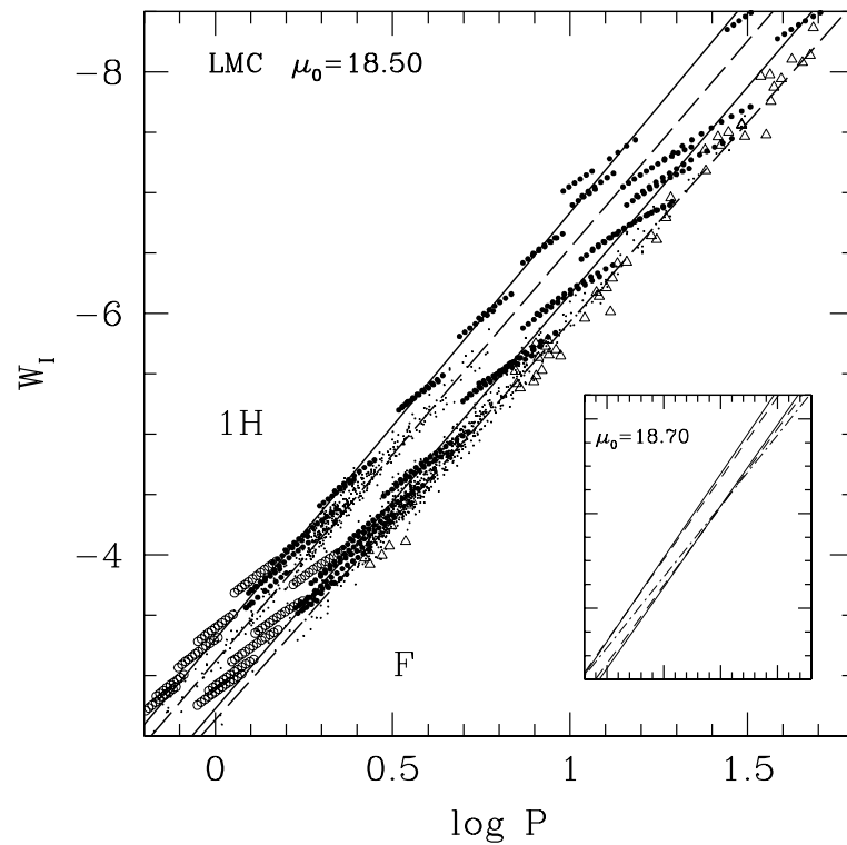
Fig. 5. \log P (in days) – W_I diagram for F and 1H pulsators for models with Z = 0.01 and LMC observed Cepheids. Symbols and curves are the same as in Fig. 3. The triangles are observations from Gieren et al. (1998). The inset displays only the mean relationships with the same linestyle as in the main figure for a distance modulus \mu_0 = 18.70 . The dash-dotted curve corresponds to the F relationship of Caputo et al. (2000)
