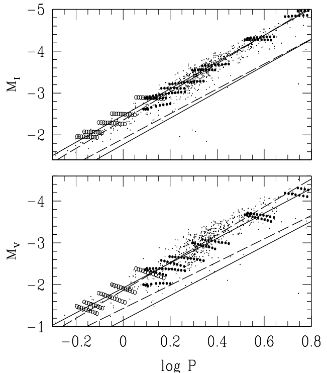
Fig. 3. Period (in days) – magnitude diagrams for 1H pulsators in the VI bands for models with Z = 0.01 and LMC observed Cepheids. The filled circles correspond to unstable 1H modes during core He burning phase from m_{\min} = 4 M_\odot to 7 M_\odot . The open circles correspond to first crossing unstable 1H modes for 3.875, 4, 4.25, 4.5, 5 M_\odot . Observations (dots) are from OGLE2 (Udalski et al. 1999a) and EROS2 (Afonso et al. 2000). The distance modulus is 18.50. The 2 solid curves are the theoretical mean PL relationships for respectively F (lower curve) and 1H (upper curve). The 2 long-dashed curves are the observed PL relationships derived by Udalski et al. (1999c) and Udalski (2000)
