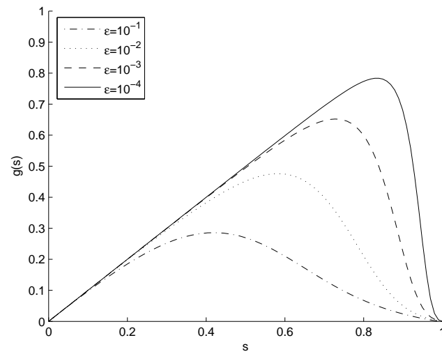
FIGURE 15. Shear contribution to the Buckley-Leverett flux function g (Case (i))
