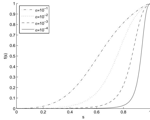
FIGURE 14. Classical contribution to the Buckley-Leverett flux function f (Cases (i) – (ii))
