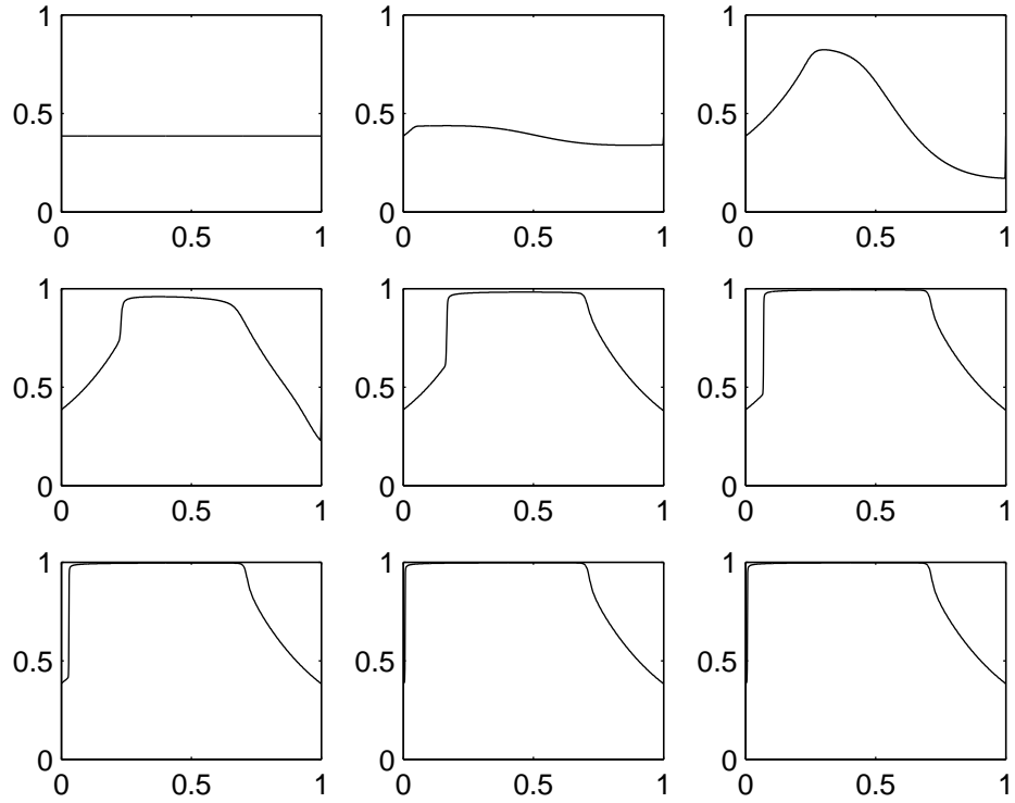
FIGURE 7. Saturation profile with partially active boundary conditions at different time steps: t = (i - 1)T_f/9 , for i = 1 to 9, from left to right, top to bottom
