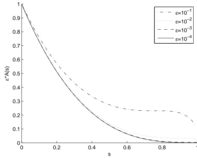
FIGURE 17. Left-hand side weight function in the Reynolds equation A (Cases (i) - (ii) )
