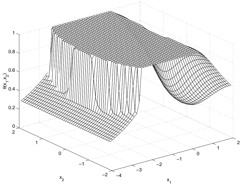
Fig. 13. Homogenized EHL saturation in the whole domain
