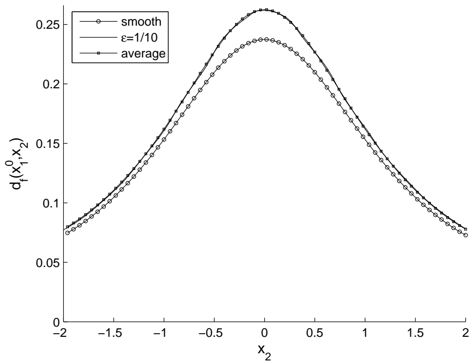
Fig. 19. EHL deformation with longitudinal patterns at x_1^0 = -0.4
