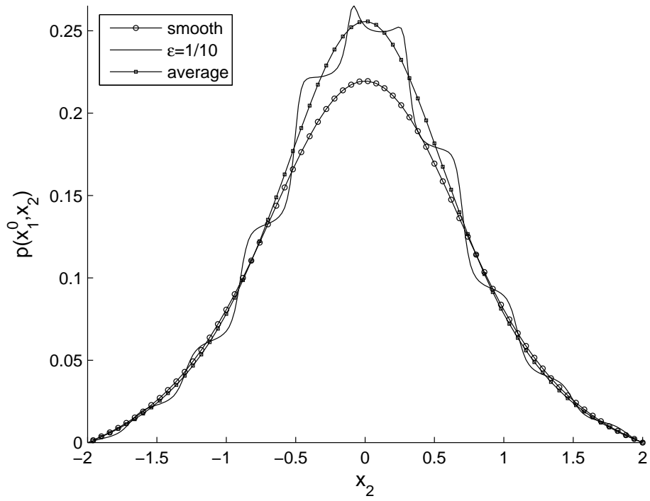
Fig. 18. EHL pressure with longitudinal patterns at x_1^0 = -0.4
