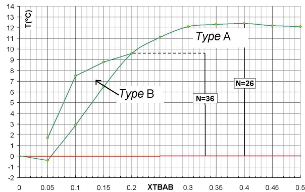
Figure 1: Experimental equilibrium diagram
