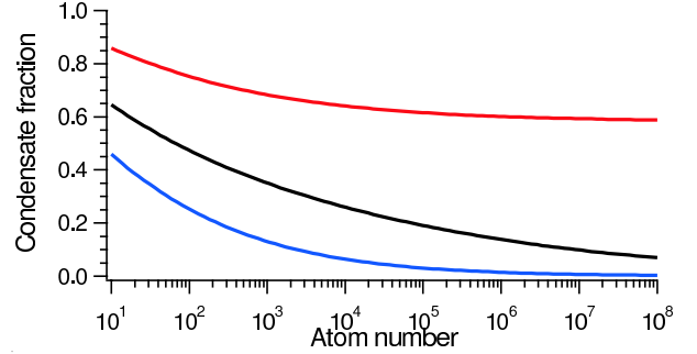
Fig. 7. Contribution of the ground-state on the peak density for, from bottom to top, 1D, 2D and 3D images in function of the number of trapped atoms. The clouds are at the transition temperature T_{ex}^* and the calculations use model ex . A 3D image would give the density in all three dimensions of space [25] whereas a 2D (resp. 1D) image corresponds to the density integrated over one (resp. 2) dimension. For N = 10^4 atoms the ground-state contributes to \sim 26\% in 2D images and \sim 6\% in 1D images. In contrast to 3D image, the ground-state contribution is very small for large atom number; it is not for typical atom numbers accessible in experiments.
