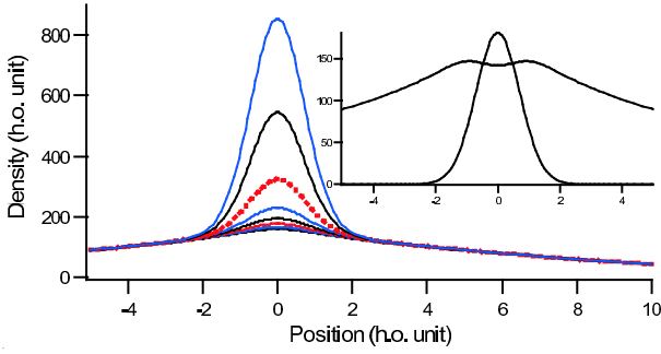
Fig. 6. Atomic density \rho_{ex} in function of r/\sigma where \sigma is the size of the harmonic oscillator ground-state. The temperature is T = 93.37\hbar\omega/k_B and the atom number N spans from 0.990 \cdot 10^6 to 1.004 \cdot 10^6 by step of 2000 atoms. The curve at threshold is in dotted line and corresponds to 10^6 atoms. The inset shows the excited states and ground state density profile at threshold. The dip around r = 0 is mainly due to the first excited state population.
