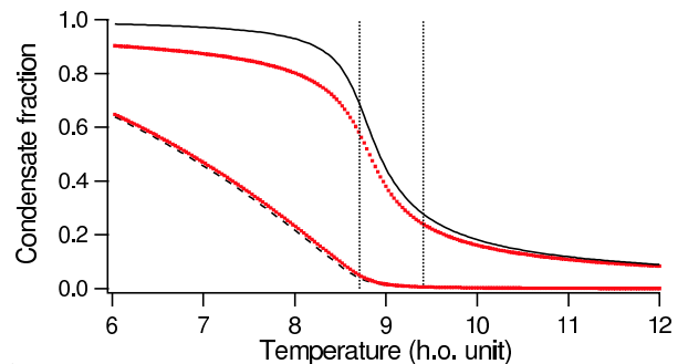
Fig. 5. Same as in Fig.4 but with 10^3 atoms. The transition temperature is T_{ex}^* = 8.71\hbar\omega/k_B and the asymptotic thermodynamic temperature is T_c = 9.41\hbar\omega/k_B . Since the number of populated states is considerably reduced compared to fig.4, the discrepancy between sc (dotted lines) and ex is more pronounced. This also explains why the increase of the condensate peak density is slower.
