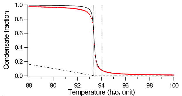
Fig. 4. Condensate atom number fraction N_0/N (dashed line) and peak density fraction \rho_0(0)/\rho(0) (solid line) in function of the temperature in harmonic oscillator unit \hbar\omega/k_B , using model ex . The cloud contains 10^6 atoms. The transition temperature is T_{ex}^* = 93.37\hbar\omega/k_B and the asymptotic thermodynamic temperature is T_c = 94.05\hbar\omega/k_B . The positions of these temperatures are shown as vertical lines in the figure. The ground-state peak density increases much more sharply than the ground-state population around the transition temperature. The former has also a significant value above T_{ex}^* . The model sc is indistinguishable for N_0/N , but is slightly different for \rho_0(0)/\rho(0) (dotted line).
