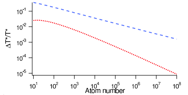
Fig. 2. Relative shift of the semi-classical transition temperatures T_c (dashed line) and T_{sc}^* (dotted line) to T_{ex}^* (see text) in function of the atom number. Both temperatures converge for high atom numbers. The critical temperature at thermodynamic limit, T_c , deviates by less than 1% for N > 5 \cdot 10^5 . The semi-classical transition temperature defined for a finite atom number, T_{sc}^* , is much more accurate and deviates by less than 1% for N > 400 .
