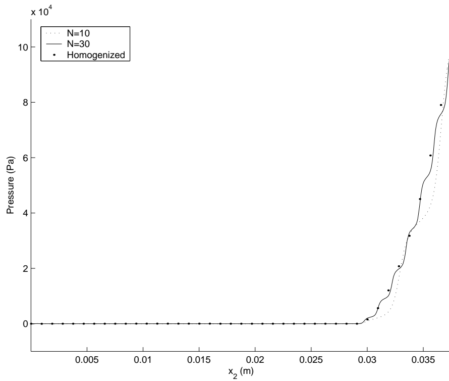
Figure 16: Hydrodynamic pressure at x_1 = 0.1060 \text{ m} (longitudinal roughness; case 2)
