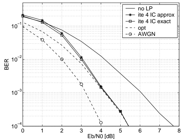
Fig. 4. BER performance of the LP-OFDM system with iterative receiver over theoretical channel with size L=4 , QPSK, 1/2-rate convolutional code, 1 bps/Hz
