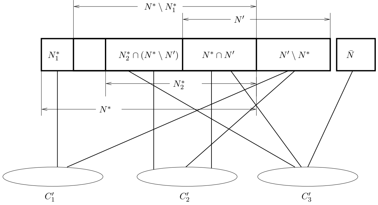
Figure 2: A rough illustration of the proof of Theorem 1.
