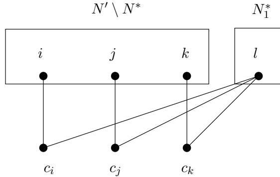
Figure 3: A connected component of B'' .
