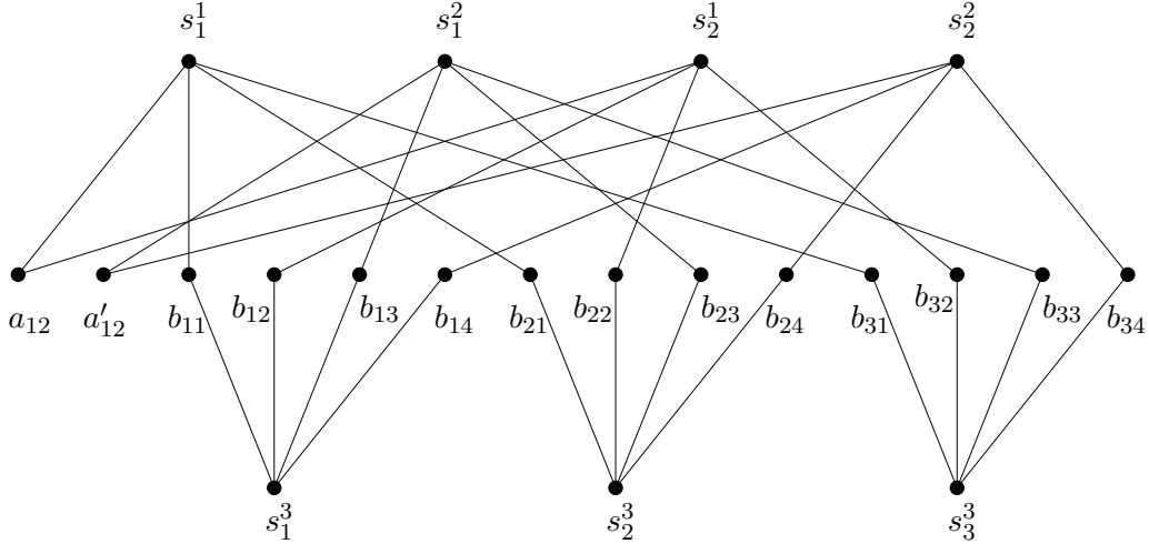
Figure 4: The characteristic graph of instance \hat{I} for \Delta = 4 .
