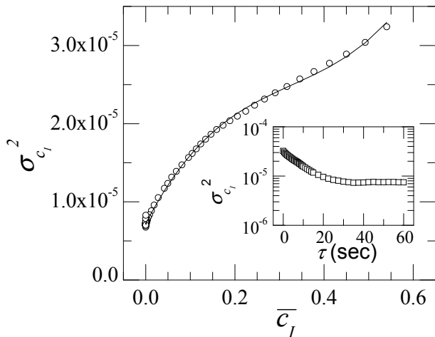
FIG. 3: Main plot: parametric representation of the variance of c_I as a function of \overline{c_I}(\tau) for the same experiment as in figs. 1 and 2 (single scattering from a dilute suspension of Brownian particles). The line is a fit of Eq. (7) to the data. Inset: same data plotted vs. \tau .
