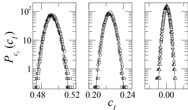
FIG. 5: Symbols: PDF of c_I(t, \tau) , P_{c_I}(c_I) , for the same suspension of Brownian particles as for the preceding figures. From left to right, the normalized delay \tau/\tau_0 is 0.09, 0.87, and 8.7. In the three panels the c_I axis spans an interval of equal width (0.04). The lines are Gaussian distributions whose mean and standard deviations are directly obtained from the c_I time series, without any fitting parameter.
