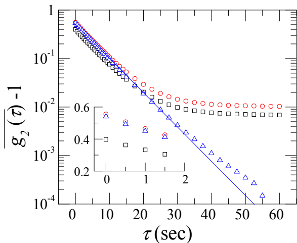
FIG. 1: Semi-logarithmic plot of the intensity time autocorrelation function measured for a suspension of monodisperse Brownian particles in the single scattering regime ( \theta = 45 deg). Data are averaged over N = 151800 pixels and over T_{\text{exp}} = 10800 sec. Squares: intensity autocorrelation function calculated from the CCD raw signal, S_p(t) ; circles: the same data after correcting for the dark noise only; triangles: after correcting for both the dark noise and the uneven detector illumination. The line is a fit to the corrected data by a single exponential decay, the functional form of \overline{g_2} - 1 predicted for monodisperse Brownian particles, yielding a characteristic time \tau_0 = 5.8 sec. Inset: zoom of the small \tau behavior of the intensity autocorrelation function.
