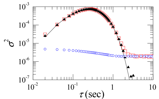
FIG. 7: Variance of c_I(t, \tau) for a foam, as a function of \tau . Open squares: variance of the raw data ( c_I ); open circles: noise contribution; solid triangles: \sigma_{g_2}^2(\tau) , the contribution due to the fluctuations of the number of rearrangement events per unit time. The line is a fit to \sigma_{g_2}^2(\tau) using Eq. (10). Data were collected in the DWS transmission geometry.
