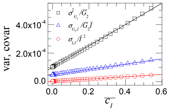
FIG. 2: Parametric plot of the normalized variance and covariance terms in the r.h.s. of Eq. (5), as a function of \overline{c_I(\tau)} , for the same experiment as in fig. 1. The lines are linear fits to the data, suggesting the c_I dependence of Eq. (6).
