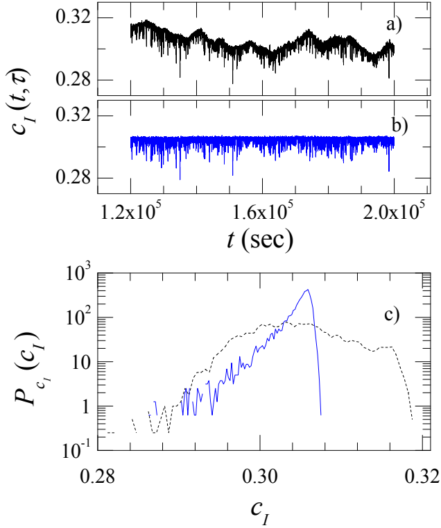
FIG. 11: a): time variation of c_I for a multilamellar vesicle gel, for \tau = 100 sec. The mean relaxation time is \tau_0 = 5050 sec, the duration of the experiment is T = 80000 sec = 15.8 \times \tau_0 . a): raw data; b): the same data after applying the correction Eq. (19); c): PDF of the traces shown in a) (dotted line) and b) (solid line).
