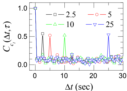
FIG. 15: Second correlation measured for a perfectly frozen speckle pattern. The curves are labelled by \tau , in sec. Note the spurious peaks at \Delta t = \tau , due to the CCD dark noise, as discussed in the text.
