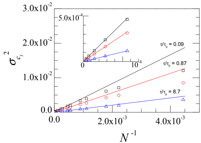
FIG. 4: For the same experiment on Brownian particles as in the preceding figures: variance of c_I as a function of the inverse number of pixels over which c_I is averaged. The lines are linear fits to the data for N^{-1} \leq 1.2 \times 10^{-4} , demonstrating that for large N \sigma_{c_I}^2 \propto N^{-1} . The inset zooms in the region near to the origin.
