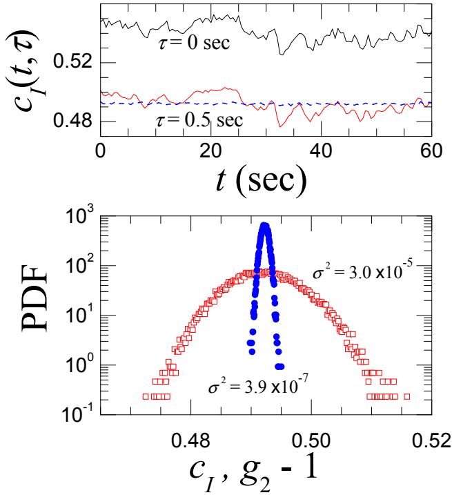
FIG. 9: Top panel: c_I(t, 0) and c_I(t, \tau_1 = 0.5 \text{ sec}) measured for a diluted suspension of Brownian particles, for which the relaxation time of \overline{g_2} - 1 is \tau_0 = 5.8 . Data are plotted over a short time window to show the strong correlation between the two traces. The dashed blue line is g_2(t, \tau_1) - 1 obtained by correcting c_I(t, \tau_1) for the noise contribution according to Eq. (19): the fluctuations due to the noise are almost completely removed. Bottom panel: PDF of c_I(t, \tau_1) (open squares) and of g_2(t, \tau_1) - 1 (solid circles), obtained over the full duration of the experiment ( T_{\text{exp}} = 10800 \text{ sec} ). The PDFs are labelled by their variance.
