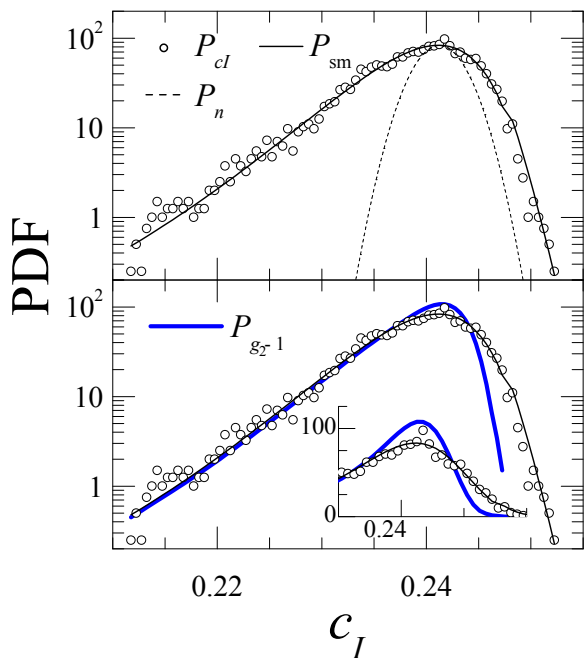
FIG. 8: Top panel: PDF of c_I(t, \tau) for a foam, for \tau = 0.2 sec (open circles); data were collected in the DWS transmission geometry. The continuous line is the smoothed distribution, P_{\text{sm}} , obtained from a fit to Eq. (16). The dotted line is the Gaussian PDF of the noise. Bottom panel: the corrected distribution, P_{g_2-1} , (thick line), together with the raw data and the smoothed PDF (same symbols as in the top panel). Note the much steeper decay of the right wing of the corrected PDF. The inset shows the data around the peak in a linear axis graph.
