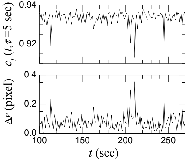
FIG. 14: Top panel: c_I(t, \tau) measured for a static scatterer, a ground glass, for \tau = 5 sec. Note the sharp drops of the degree of correlation that greatly exceed the noise of the data. Bottom panel: rigid displacement between the pair of speckle images used to calculate c_I(t, \tau) above, measured by PIV. The sharp drops of c_I are artifacts due to larger-than-average rigid shifts of the speckle images.
