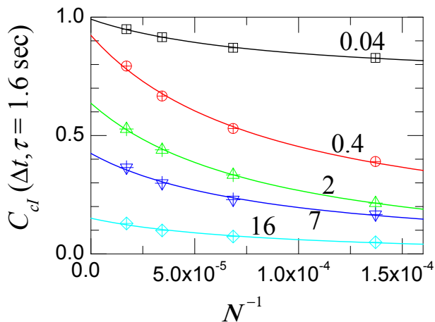
FIG. 12: Correction method for C_{g_2} . Symbols: the second correlation C_{c_I} as a function of the inverse number of processed pixels, for various \Delta t (shown by the labels, in sec) and for \tau = 1.6 sec (only the data for the largest N are shown). The data are obtained from a DWS measurement on a foam. The lines are fits to the data using Eq. (22); the full range of the fit is shown in the figure. The outcome of the fit are the values of C_{g_2}(\Delta t, \tau) and C_n(\Delta t, \tau) shown with the same symbols in fig. 13.
