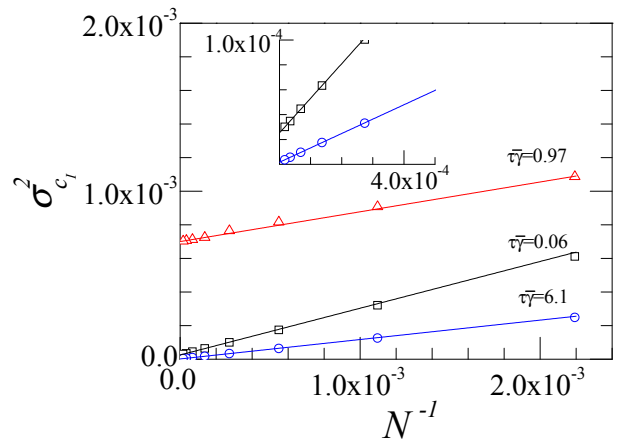
FIG. 6: Variance of c_I(t, \tau) for a foam, as a function of the inverse number of pixels over which c_I is averaged, for three time delays \tau . The lines are linear fits to the data for N^{-1} < 5.5 \times 10^{-4} . For \tau \overline{\tau} \approx 1 , the intercept of the fit strongly departs from zero, indicating temporarily heterogeneous dynamics as discussed in the text. Note that the fit yields a non-zero intercept also at small delay, as shown in the inset that zooms into the small \sigma_{c_I}^2 , large N region. Data were collected in the DWS transmission geometry for a duration T_{\text{exp}} = 160 sec, 242 times longer than the relaxation time of c_I , \overline{\tau}^{-1} = 0.33 sec.
