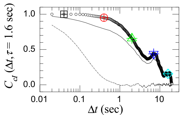
FIG. 13: Time autocorrelation function of the fluctuations of g_2 for a foam, obtained from the second correlation C_{c_I}(\Delta t, \tau) by applying the correcting scheme described in the text. Small open circles: the noise-free C_{g_2-1} ; solid line: the experimentally measured C_{c_I} ; dashed line: the noise contribution, C_n . The large symbols are the values of C_{g_2-1} obtained from the fit to the corresponding data shown in fig. 12. Note the peaks of C_{g_2-1} at \Delta t \approx 7 sec, and \Delta t \approx 14 sec, suggesting pseudoperiodic rearrangement events, as discussed in the text.
