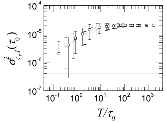
FIG. 10: Variance of c_I(t, \tau = \tau_0) calculated over a duration T as a function of T normalized by the mean relaxation time \tau_0 , for a suspension of Brownian particles. A similar behavior is observed for all \tau . The line is the contribution to the variance of c_I(t, \tau = \tau_0) of the CCD electronic noise (see the text for more details).
