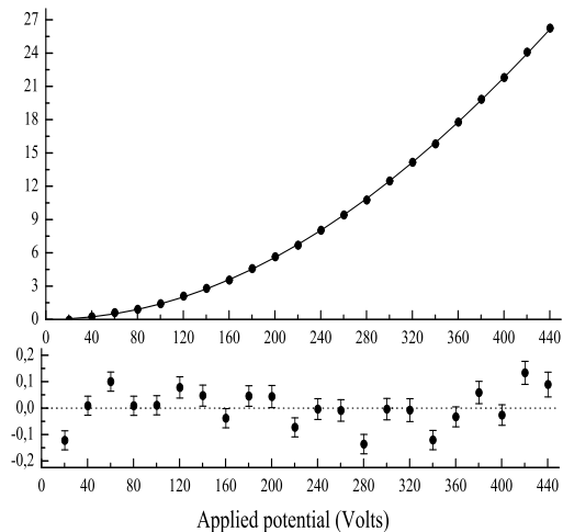
FIG. 8: The measured phase shift \phi(V_0) in radian is plotted as a function of the applied voltage V_0 : the best fit using equations (4,5) is represented by the full curve and the residuals are plotted in the lower graph with an expanded scale.
