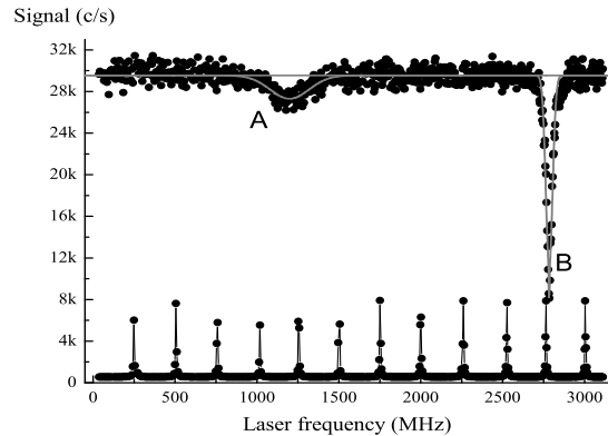
FIG. 9: Intensity losses recorded as a function of the laser frequency in MHz. The peak A corresponds to a laser beam almost contra-propagating with the atoms while the peak corresponds to laser beam perpendicular to the atomic beam. The lower curve is the transmission peaks of a Fabry-Perot confocal interferometer used for frequency calibration.
