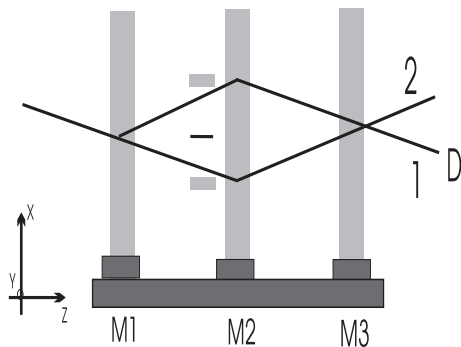
FIG. 1: Schematic drawing of our experiment based on a Mach-Zehnder atom interferometer: a collimated atomic beam, coming from the left, is diffracted by three laser standing waves made by reflecting three laser beams on the mirrors M_1 , M_2 and M_3 . The output beam labelled 1 is selected by a slit and detected by a hot-wire detector D. The capacitor with a septum between the two interfering beams is placed just before the second laser standing wave. The x , y and z axis are defined.
