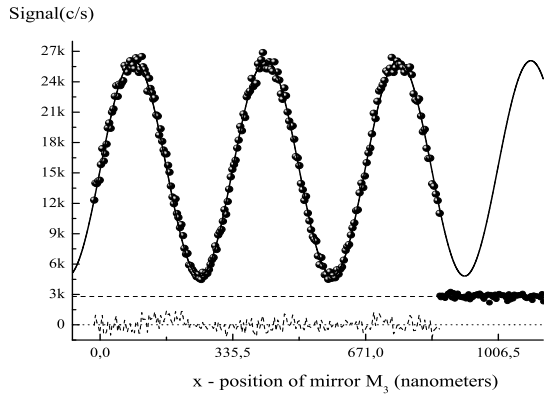
FIG. 4: Interference signal observed by displacing the mirror M_3 : the signal is expressed in counts per second, but the counting time is equal to 0.1 second only and the background signal has been recorded at the end of the experiment. The full curve is the best fit and the fit residuals are plotted, at the bottom of the figure.
