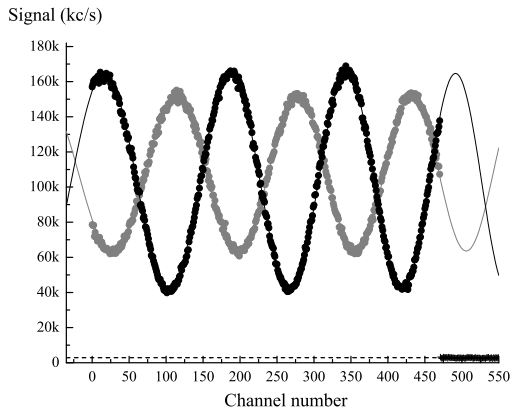
FIG. 5: Experimental signals corresponding to V_0 = 0 (black dots) and to V_0 \approx 260 Volts (grey dots). Their sinusoidal fits using equation (14) are represented by the full curves. The phase shift due to the polarizability effect is close to 3\pi and the fringe visibility is reduced because of the dispersion of the phase shift associated to the velocity spread of the lithium atoms.
