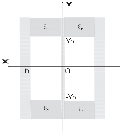
FIG. 3: Schematic drawing of the capacitor: side view. The septum in the x = 0 plane is separated from the high voltage electrodes by dielectric spacers with |y| > y_0 .
