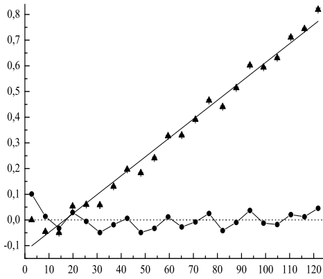
FIG. 7: The mean phase value \langle\psi_i\rangle , in radian, of the V_0 = 0 recordings is plotted as a function of the recording starting time t in minutes (with an arbitrary origin). The straight line is the best linear fit, corresponding to a phase drift of 7.5 \pm 0.2 mrad/minute. The fit residuals are also plotted and from t = 15 till t = 100 minutes, the residuals exhibit an oscillating pattern with a period close to 17 minutes.
