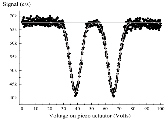
FIG. 10: Plot of the intensity of the atomic beam as a function of the voltage applied on the piezoelectric actuator inducing the rotation angle of mirror M_2 . When the Bragg condition is fulfilled, the direct beam intensity is reduced by diffraction in the diffraction orders \pm 1 . The dots represent the measured intensity and the curves their best fit. In a separate experiment, we have calibrated the rotation angle as a function of the piezo voltage, 5.83 \pm 0.03 \mu\text{rad/V} .
