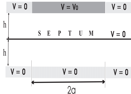
FIG. 2: Schematic drawing of the capacitor: top view. The septum is parallel to the z -axis, with the electrodes at x = \pm h . The high voltage electrodes at the V = V_0 potential extends from z = -a to z = +a , while the guard electrodes extend outside with |z| > a . The septum and the guard electrodes are at the V = 0 potential.
