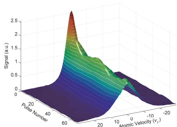
Figure 1: (color online). Experimentally measured velocity distributions as a function of time. The atomic velocity is measured in units of the recoil velocity v_r = \hbar k_L/M \simeq 3.5 mm/s. At short times, the diffusive broadening (or the reduction of the zero-velocity population) of the velocity distribution is observed. When the slowly changing perturbation is reversed (around t = 17 ), the velocity distribution starts to shrink . This is highly non-trivial behavior, showing that the destruction of dynamical localization by a slowly time-varying kick sequence is reversible. After a second cycle of the perturbation a second relocalization of the velocity distribution is observed (around t = 70 ).
