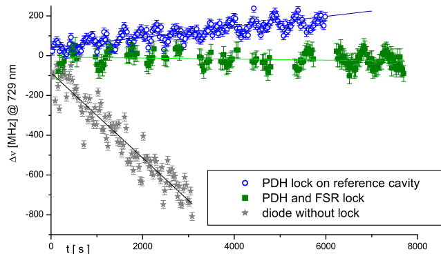
FIG. 3: Temporal evolution of the laser frequency for a free-running laser ( \star ), the laser locked by PDH method on the optical cavity ( \circ ), and with the FSR of the cavity locked on the frequency synthesizer ( \bullet ).
