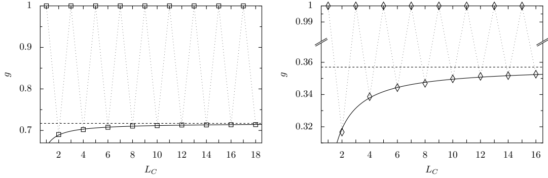
Fig. 3 – Conductance g(L_C) of the set-up sketched in Fig. 2 with L_S = 2 , for U = 1 (left) and U = 2 (right). The points are obtained with the embedding method for the ensemble. The dashed lines at g = 0.717 and g = 0.357 give the approximate values of g = |t|^4/(|t|^2 - 2)^2 , with |t| obtained by the embedding method for a single scatterer. The solid lines are fits with the forms g(L_C) = 0.7174 - 0.057/L_C for U = 1 and g(L_C) = 0.3572 - 0.077/L_C for U = 2 .
