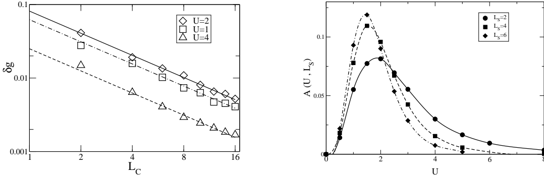
Fig. 4 – Left: Error \delta g made when using the combination law of Eq. (10) for having the conductance of the set-up sketched in Fig. 2 with L_S = 2 and different values of U , as a function of an even number L_C of connecting sites. The lines give an A(U, L_S)/L_C fit. Right: Amplitude A(U, L_S) as a function of U for different values of L_S .
