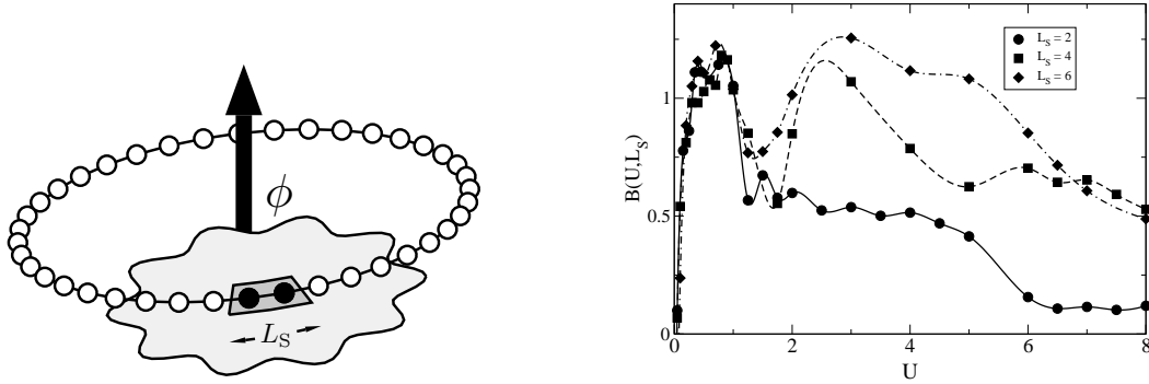
Fig. 1 – Left: Scheme of the ring pierced by a flux \phi used for the embedding method. The correlation cloud induced by L_S interacting sites upon the auxiliary lead is sketched in grey. Right: Amplitude B(U, L_S) characterizing the 1/L finite size correction to the charge stiffness.
