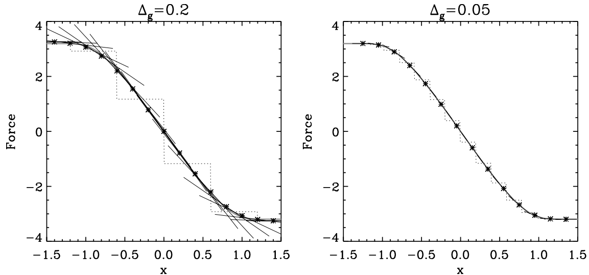
Figure 7. The calculated force for the examples considered in Fig. 4. The left- and right-hand panels correspond to the case \Delta_g = 0.2 and \Delta_g = 0.05 , respectively. On each panel, there is a smooth thick grey curve: it corresponds to the exact force derived directly from integrating equation (65). There is a thin step-like dotted curve: it corresponds to the force computed for each cell of the binary tree at the resolution needed to sample each cloud with a least N_s cells. Here we took N_s = 2 , and in practice we obtain N_{\text{inter}} = 2 or 3. There are stars nearly perfectly fitting the smooth thick grey curve: they give the force calculated at the centre of each selected cloud for doing the figure (a subset of all the clouds). A segment passes through each of these stars: it gives our weighted least-squares fit F_{\text{fit}}(x) = -2\alpha_0 x - \alpha_1 , which trivially reduces to the line passing through the two sampling points when N_{\text{inter}} = 2 . It is interesting to note that the estimate we obtain for the force at the cloud centres is very accurate, although one might notice a slight offset between symbols and the thick smooth grey line in the left-hand panel. The projected length of each segment on the x -axis is equal to the projected length of each cloud (up to cut-off). As we see, significant deviations from our local quadratic assumption are expected for the potential in the left-hand panel. These deviations are much less visible on the right-hand panel. The typical weighted deviation calculated from equation (73) by using N_s = 8 gives \Delta F/F \simeq 0.03 and 0.002 for left- and right-hand panels, respectively.
