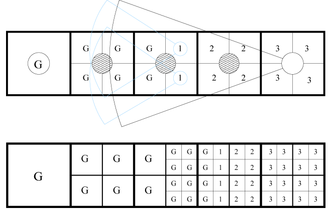
Figure B1. Sketch of our refinement procedure, for our choice of cloud size, R_L , compared to local cloud interspacing, \Delta_g/2^L : 2^L R_L/\Delta_g = \sqrt{2}/2 , which implies a 4R_L cut-off at 2^L R_{\text{max}}/\Delta_g = 2\sqrt{2} . Suppose we decide to refine the right-most cloud of the upper panel, of level L - 1 . This cloud is supplemented with four twice smaller subclouds of level L , labelled by 3. This, however, influences a region of radius R_{\text{max}}/2^{L-1} , represented by the black circular arc. To enforce our refinement criterion on all the region influenced by this cloud, we must add supplementary layers of subclouds around it, labelled by 2 and by 1. We can stop adding corrections at subclouds labelled by 1, since their extension covers the zone of influence (light circular arcs). For easy implementation of regularization (B2), we also create ghost clouds of zero mass designated by the letter ‘G’ in order to compute the correct weights for the refined level. With this refinement procedure, we see that the cloud to be refined has to be sufficiently far away from ghosts. The closest possible ghost for the right-most cloud at level L - 1 is the left-most one, which was labelled by a G surrounded by a circle. Our refinement can be performed recursively to higher level, as illustrated in the lower panel, by obeying the following simple rules: (1) it is forbidden to refine ghosts; (2) clouds labelled by 1 can only be refined in ghosts; (3) clouds labelled by 2 can only be either refined in ghosts, in subclouds labelled by 1 or in subclouds labelled by 2 according to their distance to the closest ghosts, as illustrated in the upper and lower panel; (4) clouds labelled by 3 can be fully refined. Note that, by construction, the region labelled with 3’s can be refined to arbitrary level L_\infty , while keeping smooth transitions between coarse level 0 and L_\infty .
