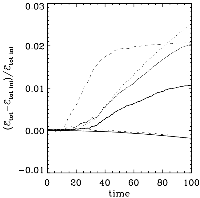
Figure 26. Energy conservation in top-hat simulations with refinement, compared to fixed-resolution simulations. The solid and dotted thin curves correspond to simulations with refinement based on local curvature and local convergence, respectively. The lower thick curve and nearly superposed dashed one correspond, respectively, to the high- and low-resolution simulations of Section 4.3. These simulations use Lucy deconvolution. The upper thick and dashed curves correspond to similar simulations, but were performed using van Citter reconstruction.
