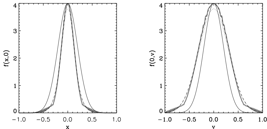
Figure 15. Comparison of the simulation with Gaussian initial conditions with a stationary solution. The function f(x, 0) is displayed in the left-hand panel, while the function f(0, v) is displayed in the right-hand panel. On each panel, the simulation (thick grey curve) is compared to the stationary solution given by equation (87) with the same energy and same mass (dots). The dashes are the same as the dots, except that the stationary solution has been normalized to match the maximum of f . For reference, the thin solid curve corresponds to initial conditions.
