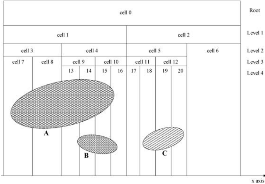
Figure 6. Sketch of our tree structure used to compute the forces within each cloud. Here, we consider the case N_s = 3 , i.e. each cloud must intersect with at least three cells of the tree at a given refinement level. Note that for computing the forces for cloud A, only cells 7, 8, 9 and 10 of level 3 of refinement will be used, even if more refinement is available due to cloud B.
