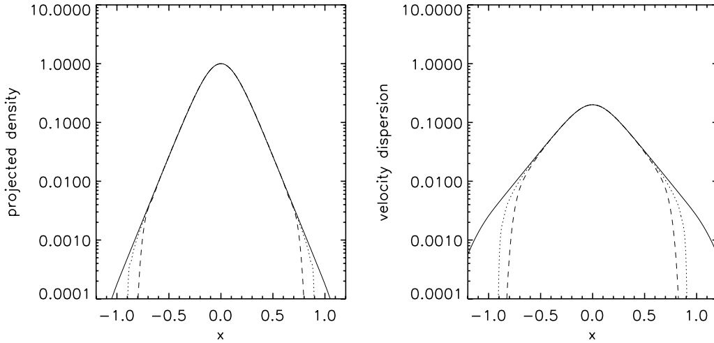
Figure 11. Mean projected density, \rho(x) = \int f(x, v) dv (left-hand panel) and velocity dispersion, v_{\text{rms}}(x), v_{\text{rms}}^2(x) \equiv \langle \delta v^2 \rangle = \int f(x, v) v^2 dv - [\int f(x, v) v dv]^2 (right-hand panel), as functions of position, for the stationary solution examined in Fig. 10. The solid curve corresponds to equation (87) with apodization as described in the text, which explains the bending of the tails visible in the right-hand panel. The dotted and the dashed curves give the results obtained from the high- and the low-resolution simulations, respectively.
