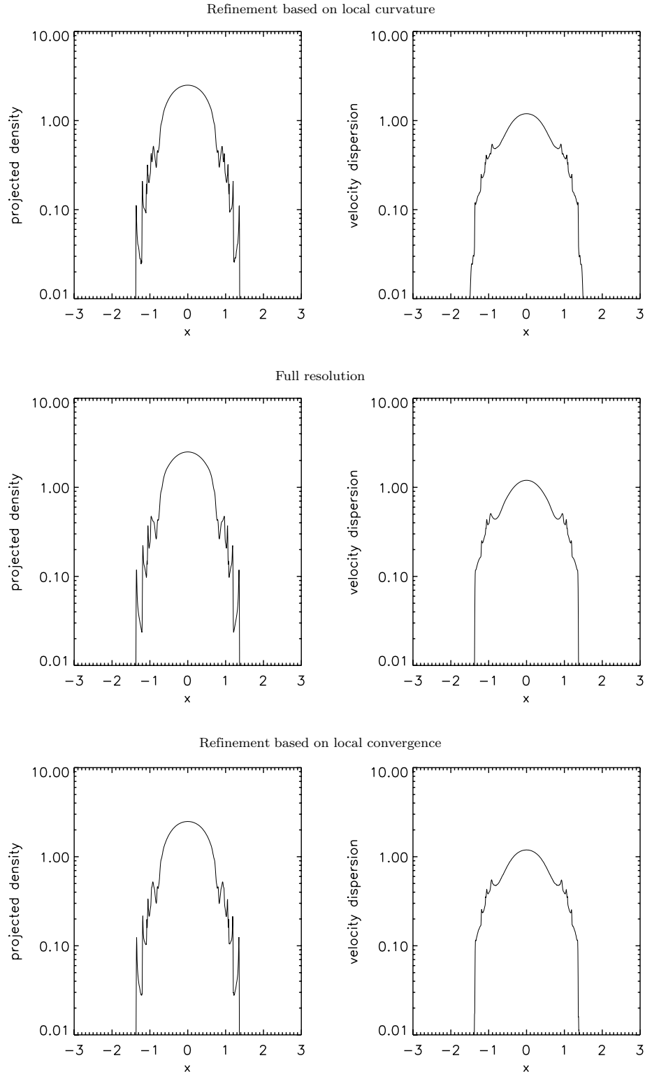
Figure 24. Mean projected density (left-hand panels) and velocity dispersion (right-hand panels), as functions of position, for top-hat simulations with refinement based on local curvature (top row) and on local convergence (bottom row), compared to full resolution (middle row), at t = 40 .
