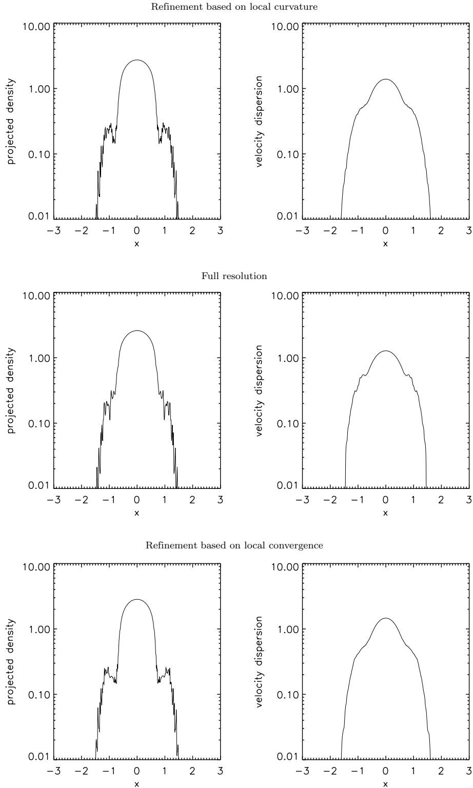
Figure 25. Same as Fig. 24, but for t = 100 .
