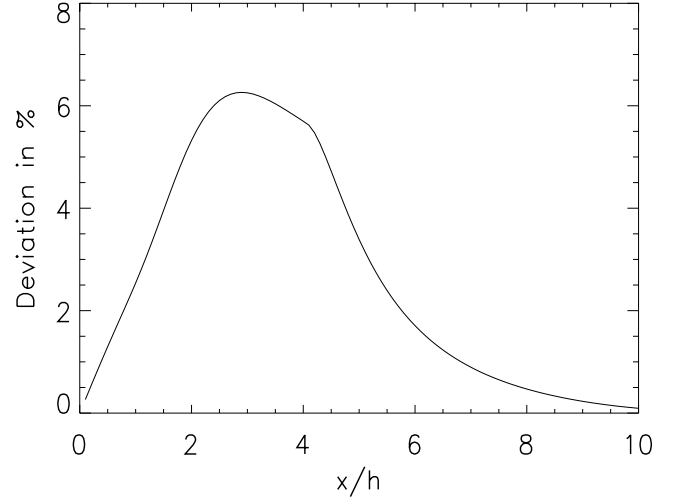
Figure 1. The maximum deviation from the quadratic approximation as a function of the initial position x_0 . The distribution has a scalelength h 10 times larger than the cloud. The coordinate x_0 has been normalized by the scalelength of the distribution h . Note that the maximum deviation is at about 3h from the centre of the distribution.
