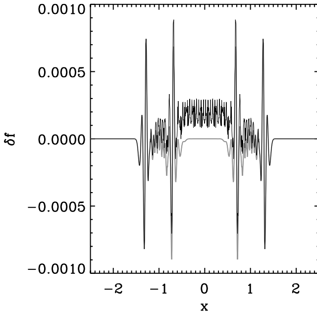
Figure 5. The difference \delta f(x, 0) as a function of x , between the reconstructed (with van Citter) and true distribution function, whether equation (59) (thin black curve) or equation (66) is used to compute \tilde{f} . The function f to sample is the same as in Fig. 4 and the resolution is the same as in the lower panels of this figure.
