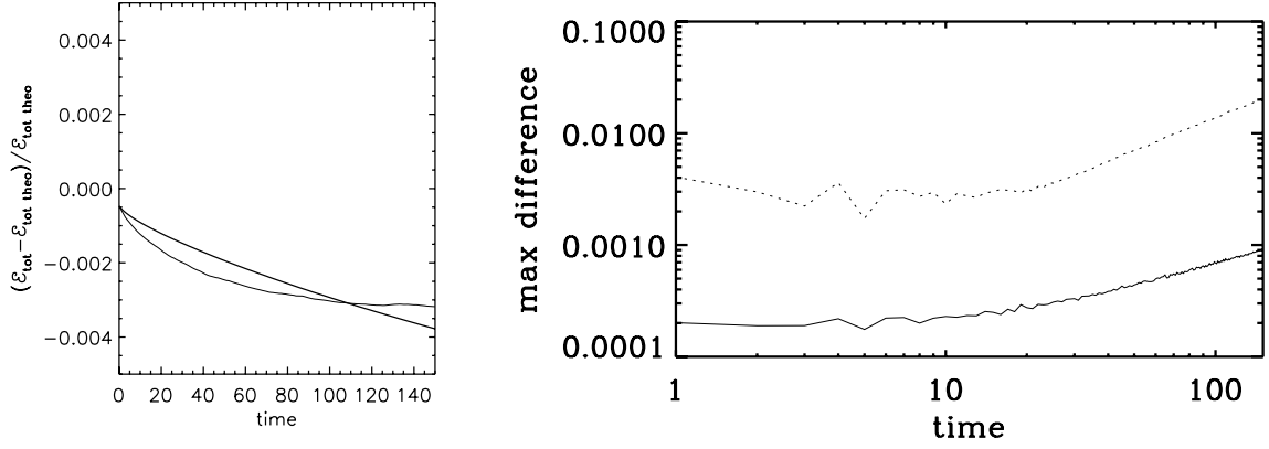
Figure 10. Left-hand panel: test of energy conservation for a stationary solution: The quantity (\mathcal{E}_{\text{tot}} - \mathcal{E}_{\text{tot,theo}}) / \mathcal{E}_{\text{tot,theo}} is displayed as a function of time, where \mathcal{E}_{\text{tot}} is measured in our simulation according to equation (83) and \mathcal{E}_{\text{tot,theo}} is given by equation (90). The parameters used to do the simulations are \bar{\rho} = 2 and \sigma_v = 0.2 . The thick and the thin curves correspond to the high- and the low-resolution simulations, respectively. Right-hand panel: deviations from stationarity: the quantity \max |\tilde{f}(x, v, t) - f_s(x, v)| is represented as a function of time, where \tilde{f} is the simulated f and f_s(x, v) is given by equation (87) with additional apodization as explained in the text. The continuous and the dotted curve correspond to the high- and the low-resolution simulations, respectively.
