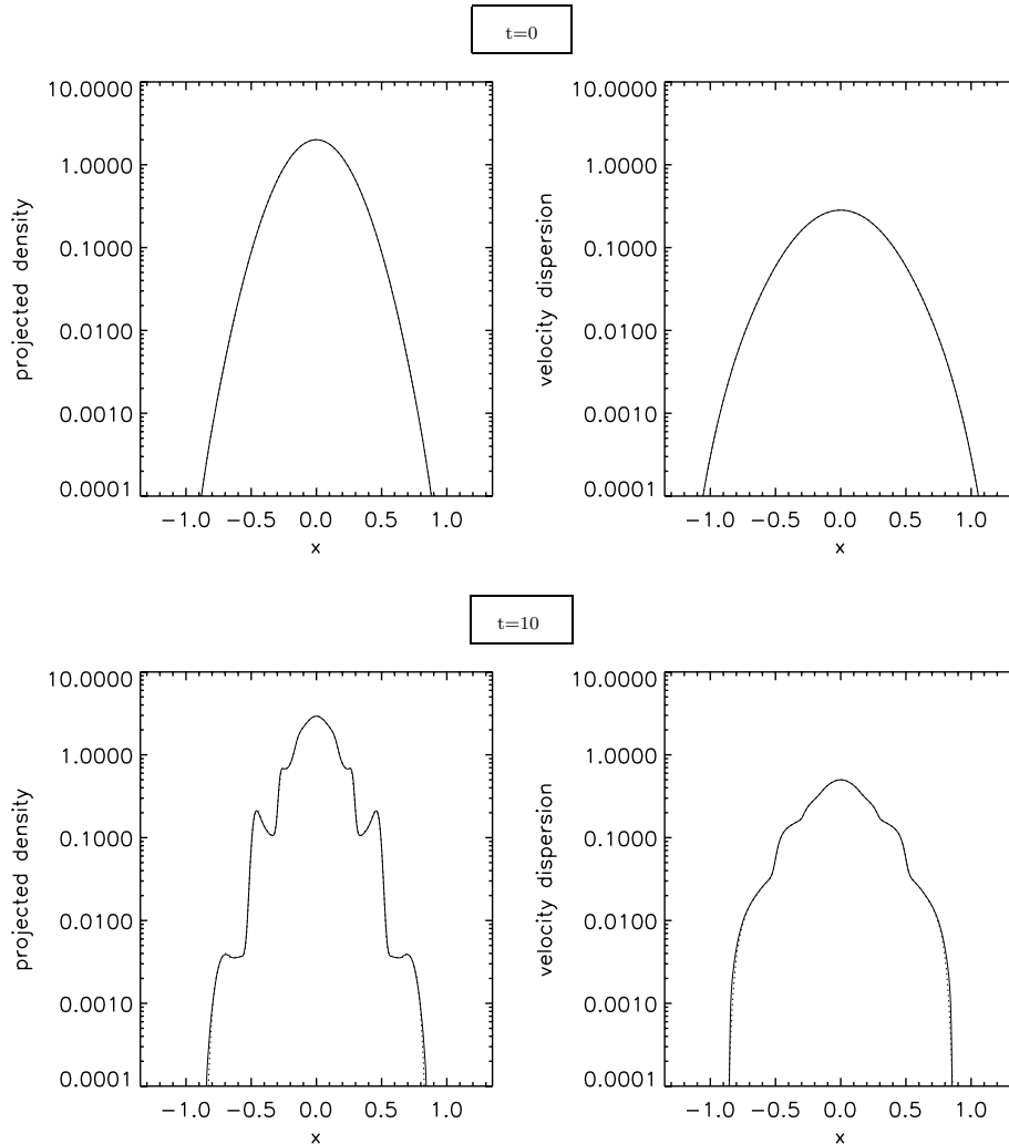
Figure 13. Mean projected density (left-hand panels) and velocity dispersion (right-hand panels), as functions of position, for the simulations with Gaussian initial conditions. Each row of panels corresponds to a given time. The solid curve and the dotted curve are for the high- and the low-resolution simulations, respectively, except for t = 0 : in that case, the curves are calculated according to equation (84).
