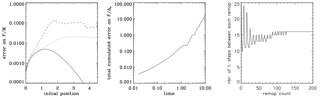
Figure 8. Left-hand panel: the maximum instantaneous error, \Delta F/F_{\text{max}} , in the force calculation (equation 73) as a function of initial cloud position, measured in a simulation without remapping. The initial conditions considered here are a truncated Gaussian of size \mathcal{R} as given by equation (84). The initial position, x_{\text{ini}} , of the cloud is expressed in units of h . To reproduce a case similar to the one studied in Fig. 1, the cloud size R is given by R/h = 0.1 . Three dynamical times are considered, t = 0.5 (solid), 1.5 (dots) and 6.0 (dashes). It is difficult to make an exact comparison to Fig. 1, given that fact that our estimate of \Delta F/F_{\text{max}} is a quadratic dispersion. However, the general order of magnitude found on the error agrees with the results of Section 2.2.4. The dotted curve which corresponds approximately, dynamically, to the parameters chosen to make Fig. 1, agrees well, at least qualitatively with Fig. 1. Middle panel: the maximum cumulated error, E_{\text{cum}/\Delta_v}^{\text{max}} , as a function of time. A remapping should be performed each time this error exceeds some threshold. Right-hand panel: the number of time-steps, n_{\text{remap}} , between each remap as a function of remap count, when the condition (85) is fulfilled, with E_{\text{max}} = 0.05 . The simulation used to make this plot is exactly the same as the one used for the left-hand and middle panels, except that Lagrange remap was enforced. The simulation was stopped after 3000 time-steps, at t \simeq 39 , corresponding to 35 dynamical times according to equation (37) with \rho_0 = \bar{\rho} . Note that the variations of n_{\text{remap}} decrease with time: n_{\text{remap}} seems to converge progressively to some fixed value, as expected, while the system relaxes to a stationary state.
