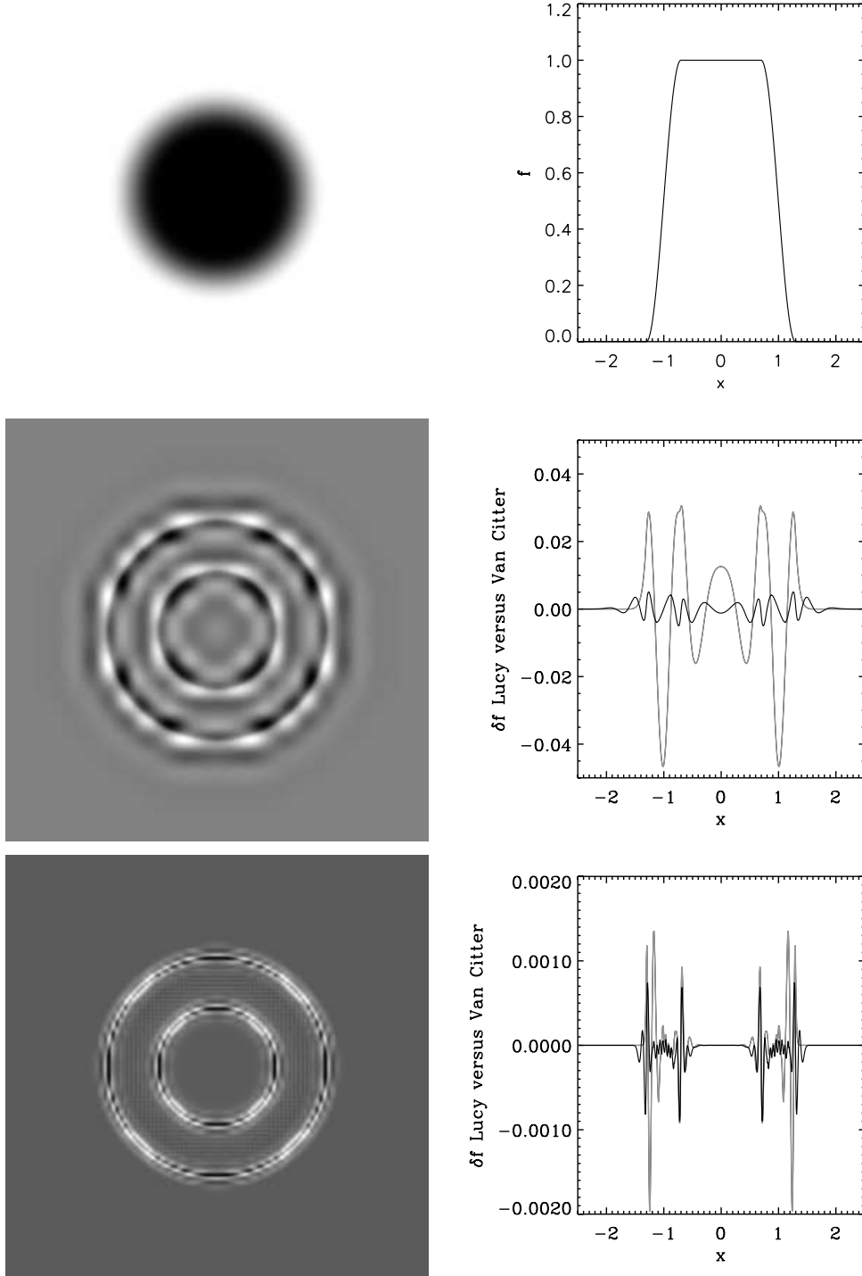
Figure 4. Comparison of the van Citter and Lucy algorithms for reconstructing a distribution in phase space. The upper left-hand panel displays the function f(x, v) we aim to reproduce, as given by equation (65) [darker regions correspond to larger values of f(x, v) ]. The upper right-hand panel shows f(x, 0) as a function of x . The middle left-hand panel displays \delta f \equiv \tilde{f} - f , where \tilde{f} is obtained by using the van Citter algorithm. A very similar result would be obtained for Lucy. The middle right-hand panel gives \delta f(x, 0) as a function of x , both for van Citter (thin black curve) and Lucy (thick grey curve). To sample the distribution function, an interspacing of \Delta_g = 0.2 and a cut-off R_{\max} = 3.95\Delta_x was used. The lower left- and right-hand panels are the same but for higher resolution, \Delta_g = 0.05 . Note that, for the four lowest panels, the weighting scheme discussed in Section 3.1.3 has been used to estimate \tilde{f} , following equation (66).
