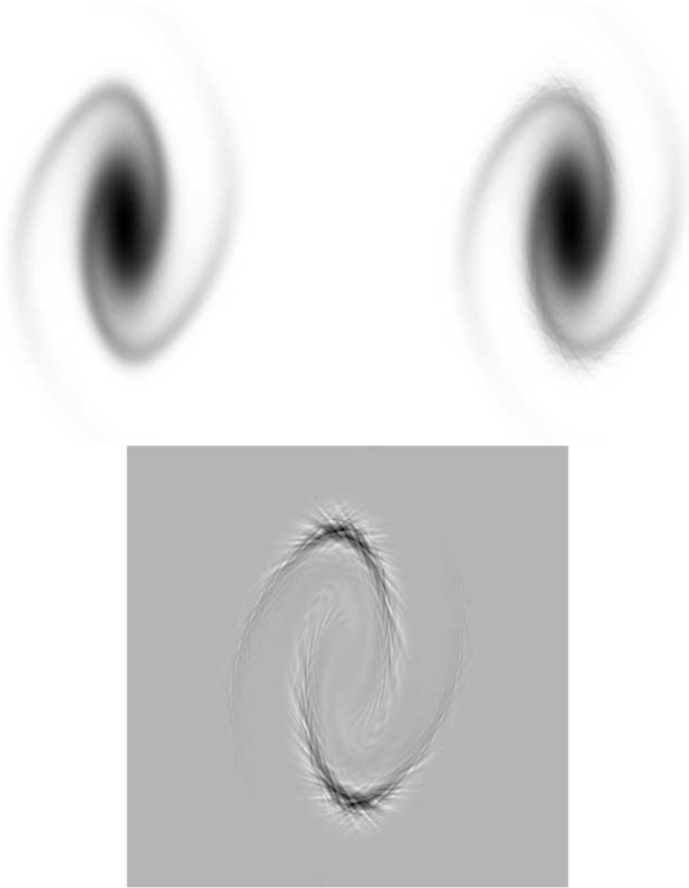
Figure 9. Apparition of a hairy structure after a few dynamical times. The simulation considered is the same as the one in the two left-hand panels of Fig. 8, at t = 6 . The top left-hand panel gives the ‘correct’ answer, i.e. f(x, v) obtained by remapping the density field with new round clouds using condition (85) with E_{\max} = 0.05 . The top right-hand panel shows the ‘wrong’ answer obtained without remapping. The bottom panel displays the difference between left- and right-hand panels, which shows the hairy structure appearing due to the divergence of the axis ratios of the clouds.
