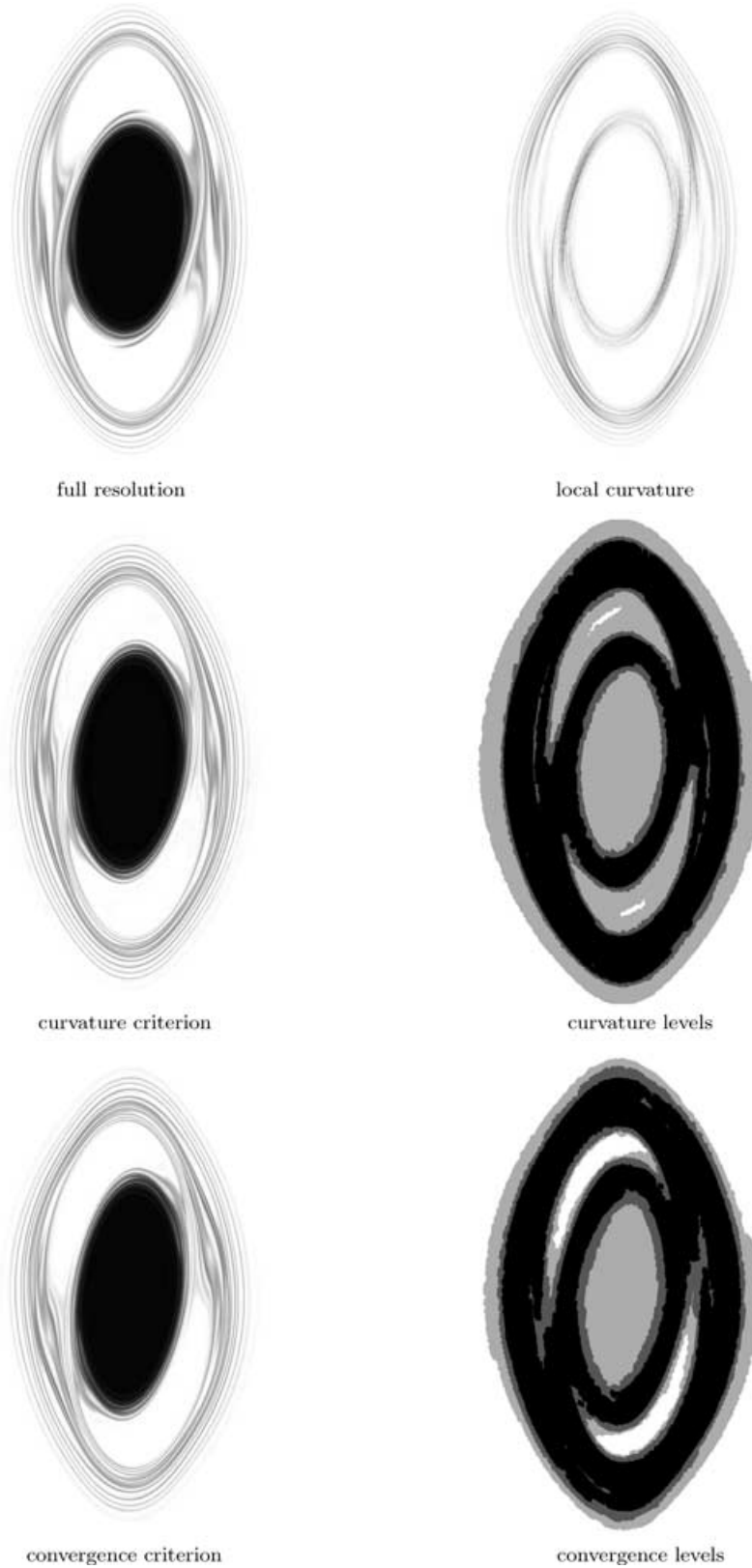
Figure 23. Same as in Fig. 21, but for t = 100 .
