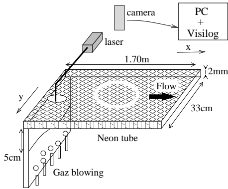
Fig. 1. Schematic drawing of the set-up from which we collected the experimental results [1] referred to in the present theoretical paper.
