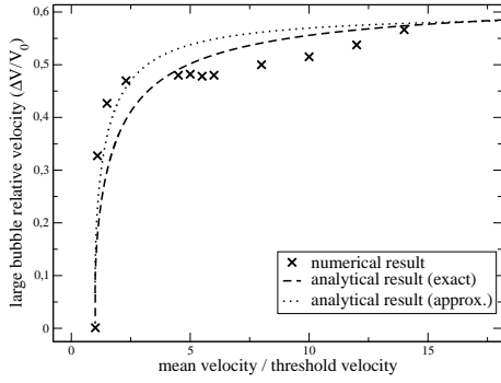
Fig. 13. Large bubble relative velocity as a function of the mean flow velocity. The first analytical law is given by eq. 45 and the second one comes from eq. 31. Numerical prefactors are adjusted to obtain the best fit between numerical and analytical values. Their values are respectively 0.25 and 0.2, which is of the order of unity as expected. The ratio D/d is 3.
