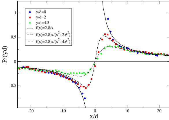
Fig. 16. Pressure field in the foam after removing the equilibrium and linear contributions. The foam flows from the left ( x < 0 ) to the right ( x > 0 ). (a) Numerical results. Light gray corresponds to high pressure values. (b) Another view of the same results : pressure in the foam along the line y = \text{const.} , for three value of y . The line y=0 goes from upstream to downstream, trough the middle of LB. The values are well fitted by the analytical expression 34.
