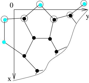
Fig. 6. The encircled vertices belong to the line \mathcal{L} . Their velocities are fixed to a given value to impose the flow rate. The two axes are sides of the simulation box, gray vertices result from the use of periodic boundary conditions.
