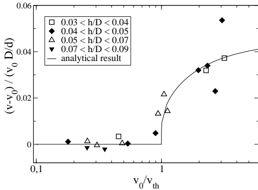
Fig. 14. Experimental results from Cantat et al. [1]. Large bubble relative velocity as a function of the mean flow velocity, rescaled by the threshold velocity obtained on Fig.10, for various large bubble sizes. The analytical fit comes from eq. 31, with a single adjustable prefactor.
