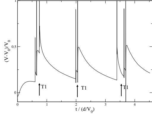
Fig. 12. Numerical LB velocity as a function of time, for v_0 > v_{th} . T1's involving LB edges occur in avalanches of 2 or 3 events and are indicated by arrows. At these times the LB is suddenly deformed and the center of mass velocity diverges numerically. Just after a T1 avalanche, the elastic stress is strongly reduced and the LB velocity is large. As the stress accumulates in the small bubbles network the LB velocity decreases until the yield stress is reached and new plastic events occur. In contrast, if v_0 < v_{th} the LB relative velocity tends to zero before the yield stress is reached.
