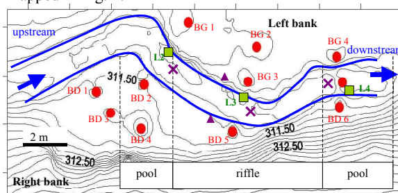
Figure 1. locations of the geomorphologic features and the different measurement devices. Solid lines delimit the streambed. \times Cluster of 3 micropiezometers in the streambed (15, 30 & 50 cm deep); BG: Piezometer in the banks; L: Free surface water level measurement devices; \blacktriangle : Tensiometers.
