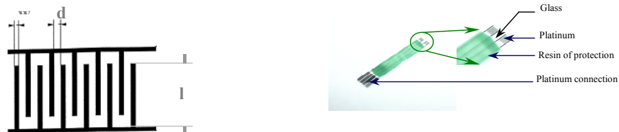
Figure 1: Design of one pair of interdigitated electrodes and photograph of the transducer. The width ( w ) of the digits and the interdigitated distance ( d ) are both 10 \mu\text{m} . The digits are 900 \mu\text{m} long ( l ). Thus, the sensitive area of the device is about 1.6 \text{ mm}^2 .
