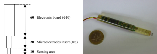
Figure 1 : design of the micro-sensor
