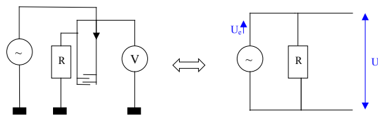
Figure 2: schematic wiring and equivalent circuit
