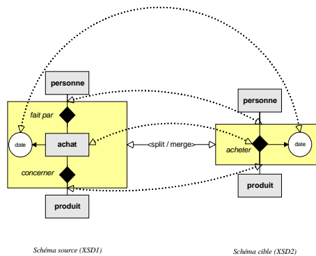
2 relations & 1 concept \ll 1 relation (a) \text{merge}\{achat \& \text{fait par} \& \text{concerner}\} @ \text{acheter} ; XSD_1 @ XSD_2, \bar{n} (b) \text{split}\{acheter\} @ \{achat \& \text{fait par} \& \text{concerner}\} ; XSD_2 @ XSD_1, \bar{n}
