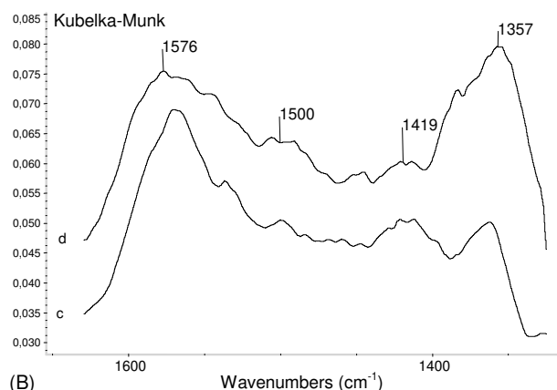
Fig. 7. DRIFT spectra of Co/35 wt.% MgO-SiO 2 , recorded at 600 °C: (a) under flowing He; (b) under flowing CH 4 /He = 10/90 vol.%; (c) under flowing CO 2 /He = 10/90 vol.% and (d) under flowing reacting mixture CH 4 /CO 2 /He = 10/10/80 vol.%.
