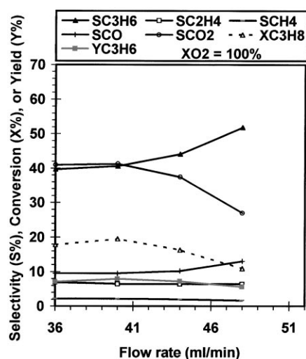
Fig. 10. C_3H_6 , C_2H_6 , C_2H_4 , CH_4 , CO , CO_2 selectivities; C_3H_8 conversion and propene yield for the V-MFI membrane as a function of the total flow rate. The O_2 conversion was always 100% with flow-through contactor configuration for feed composition 6% C_3H_8 and 1% O_2 in He at temperature 550^\circ C .
