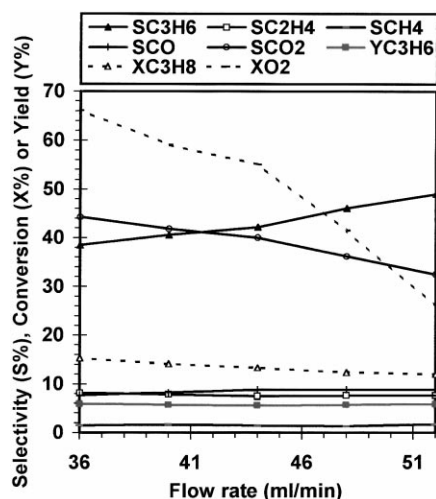
Fig. 9. C_3H_6 , C_2H_6 , C_2H_4 , CH_4 , CO , CO_2 selectivities; C_3H_8 and O_2 conversions and propene yield for the MFI membrane as a function of the total flow rate with flow-through contactor configuration for feed composition of 6% C_3H_8 and 1% O_2 in He at temperature 550^\circ C .
