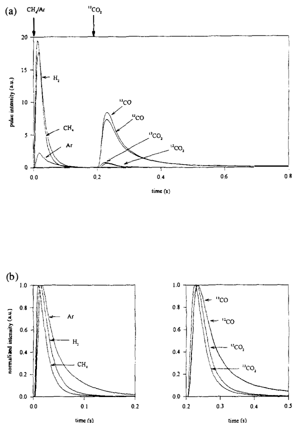
Fig. 5. (a) TAP pump-probe pulse responses using 12 CH 4 and 13 CO 2 at 550°C over Ru/SiO 2 (b) Normalised responses.
