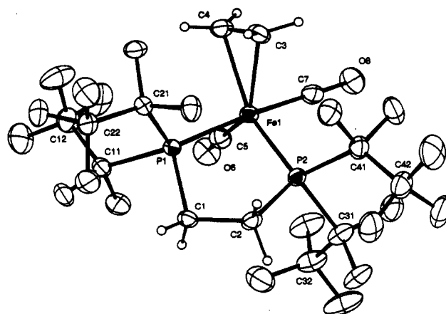
Figure 1. ORTEP diagram of (\text{dfep})(\text{CO})_2\text{Fe}(\eta^2\text{-CH}_2=\text{CH}_2) .
