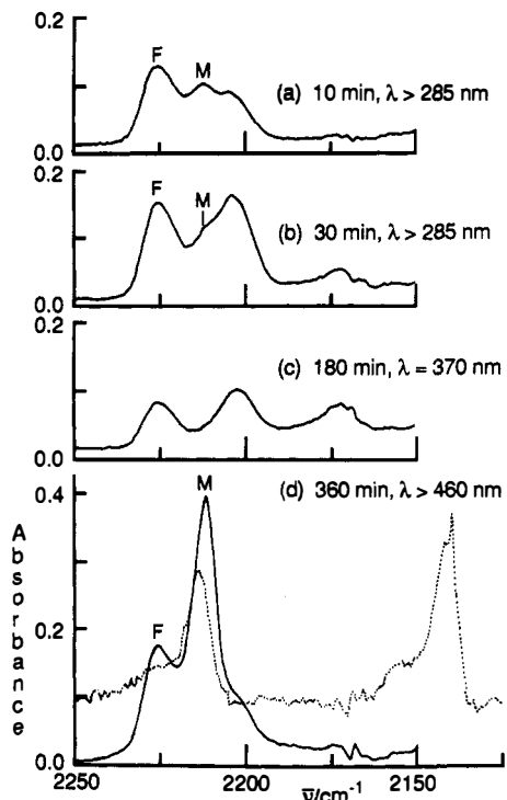
Figure 5. (a) IR spectrum in the N-N stretching region observed following 10 min photolysis of 1 in a 5% N 2 /Ar matrix at 12 K (2.5 h deposition, sample at 293 K, window at 20 K, 4.9 mmol of gas deposited); (b) spectrum after a total of 30 min photolysis (λ > 285 nm); (c) spectrum after 180 min photolysis with λ = 370 nm which is selective for the dinitrogen products; (d) full line, spectrum after 360 min photolysis with λ > 460 nm which selects (Ar)Cr(CO) 3 (dfepc): F = fac -(N 2 )Cr(CO) 3 (dfepc); M = mer -(N 2 )Cr(CO) 3 (dfepc); dotted line, spectrum at the corresponding stage of an experiment with 1 in 14 N 2 / 15 N 2 /Ar (2.5:2.5:95). The remaining bands illustrated are probably due to (N 2 ) 2 Cr(CO) 2 (dfepc). These spectra correspond exactly to the UV-vis spectra in Figure 6.
