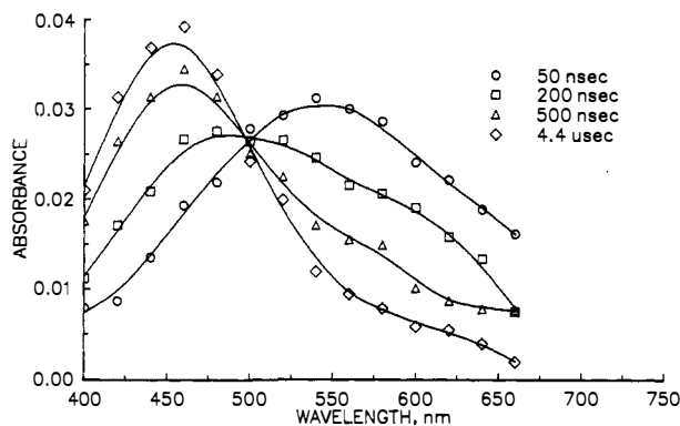
Figure 9. Photolysis ( \lambda = 355 \text{ nm} ) of 1 (ca. 2 mM) with 6 mM Et 3 SiH in dry, degassed, dry hexane.
