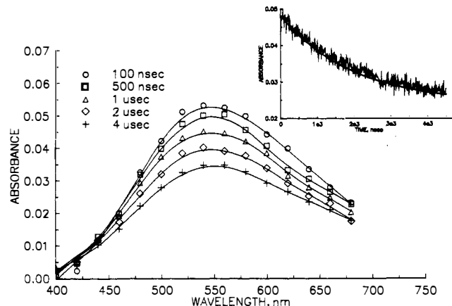
Figure 7. Photolysis (λ = 355 nm) of 1 (ca. 2 mM) in degassed, dry hexane. The inset shows exponential and a constant using the rates in Table II.
