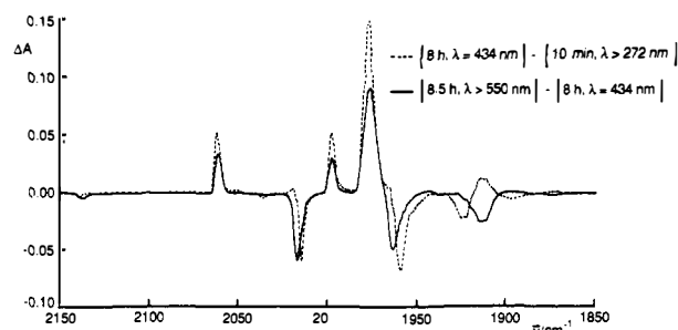
Figure 3. IR difference spectra in the \nu(\text{CO}) region showing the effect of selective photolysis on 1 in a methane matrix. Initial photolysis for 20 min with \lambda > 272 nm (a) was followed by 8 h photolysis with \lambda = 434 nm (b) and then 8.5 h photolysis with \lambda > 550 nm (c): broken line, b-a; full line, c-b.
