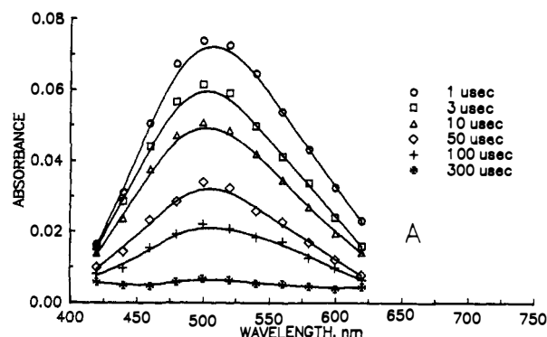
Figure 14. Decay of the slow components from the irradiation ( \lambda = 355 nm) of 2 (ca. 2 mM): A, in dry, degassed hexane; B, in dry hexane saturated with CO.
