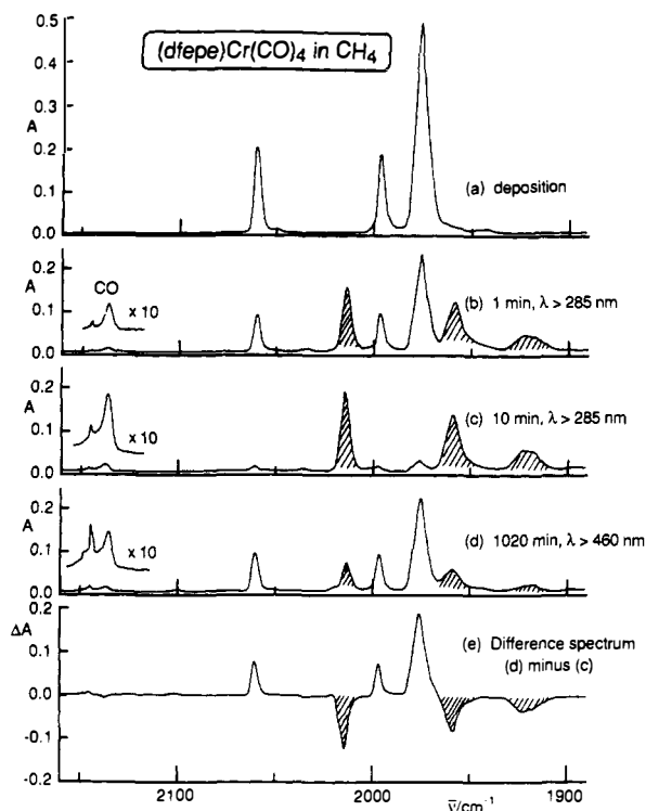
Figure 1. (a) IR spectrum in the CO stretching region of 1 in a methane matrix at 12 K (1 h deposition; sample temperature, 293 K; matrix temperature, 20 K; 1.6 mmol CH 4 deposited). (b) Spectrum after 1 min of mercury arc photolysis ( \lambda > 285 nm) showing depletion of 1 , release of CO, and growth of fac -Cr(CO) 3 (dfepe) (shaded). (c) Spectrum after a total of 10 min of photolysis ( \lambda > 285 nm). (d) Spectrum after a further 1020 min of photolysis ( \lambda > 460 nm) designed to irradiate into visible absorption band of the product. (e) Difference spectrum calculated as spectrum d minus spectrum c showing regeneration of 1 and loss of product.
