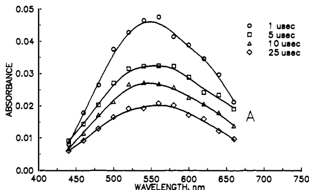
Figure 13. Decay of the slow components from the irradiation ( \lambda = 355 nm) of 1 (ca. 2 mM): A, in dry, degassed hexane; B, in dry hexane saturated with CO.
