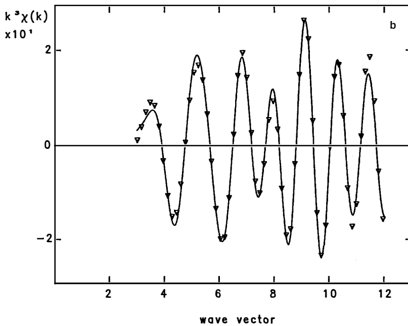
Fig. 4. Experimental (triangles) and modeled (full line) EXAFS contributions around a platinum atom: a-sample B; b-sample B s .
