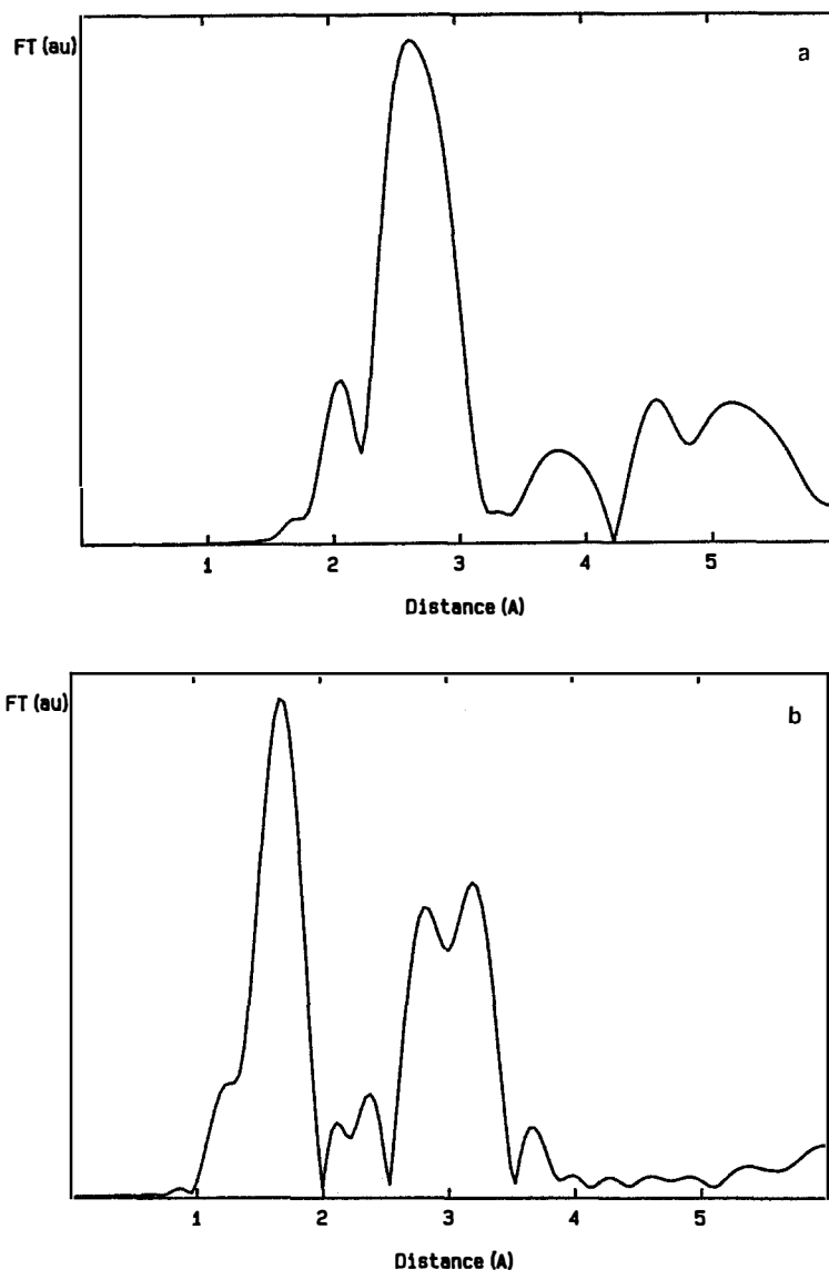
Fig. 3. Radial distribution functions obtained by Fourier transforming the data shown in fig. 2. The vertical bars mark the selected range in R to compute the inverse Fourier transform.
