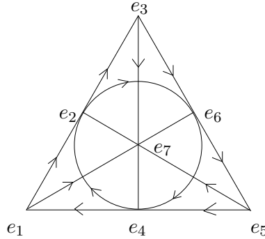
Figure 1. Octonionic multiplication
