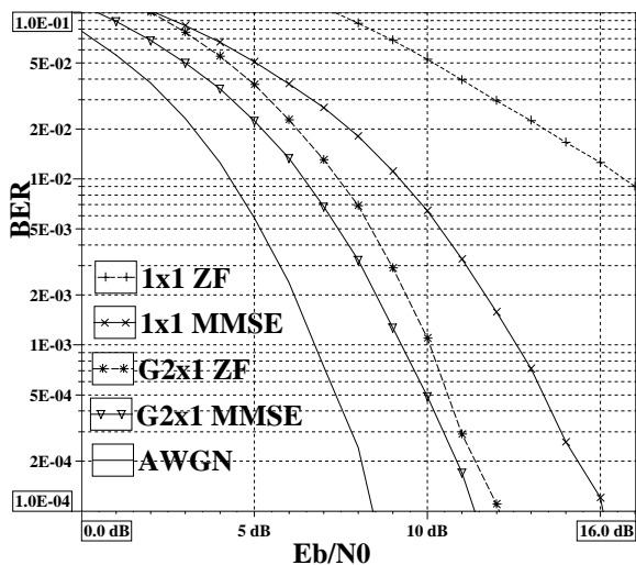
Fig. 3. MMSE and ZF SD performance over Rayleigh channel for SISO and Alamouti MISO MC-CDMA systems.
