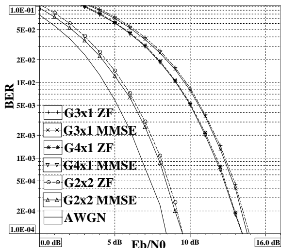
Fig. 4. Single-user MMSE and ZF SD performance over Rayleigh channel for STBC MC-CDMA systems offering a 2 bps/Hz spectrum efficiency
