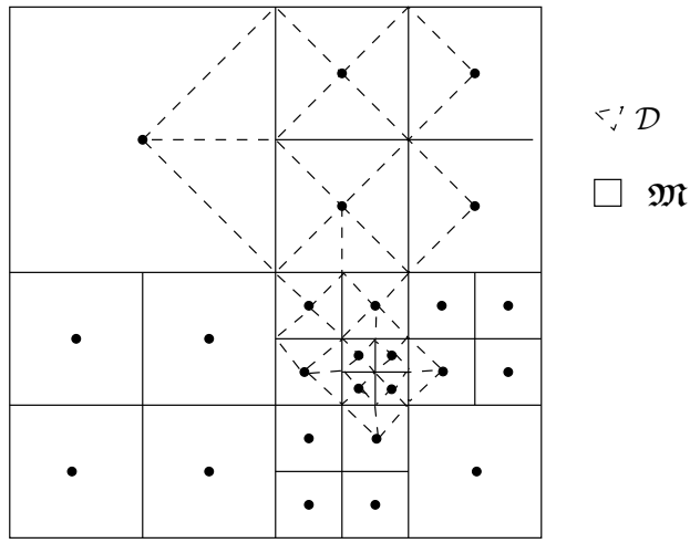
FIG. 2.4. Local refinement allowed by the boundedness of \text{reg}(T)
