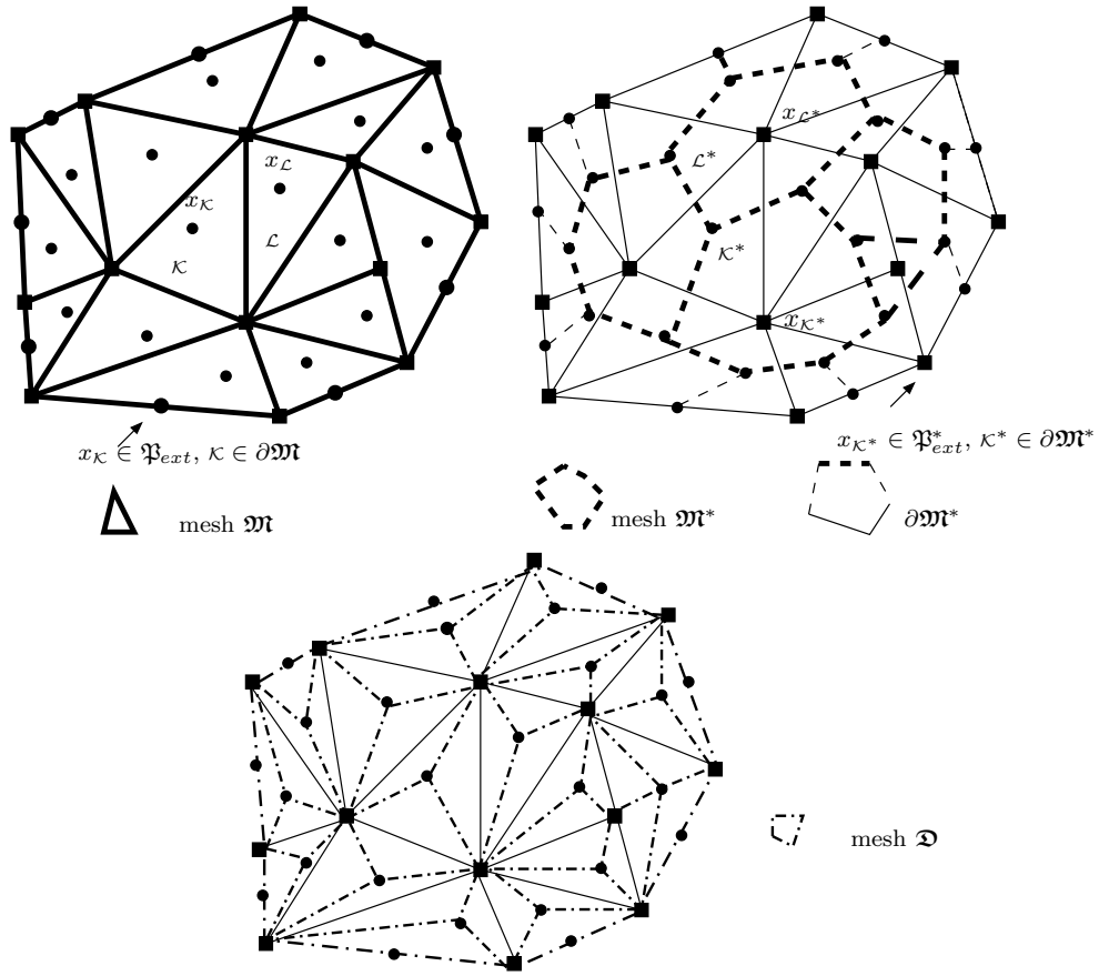
FIG. 2.1. Example of a DDFV mesh
