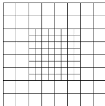
FIG. 8.1. Picture of the mesh 1
