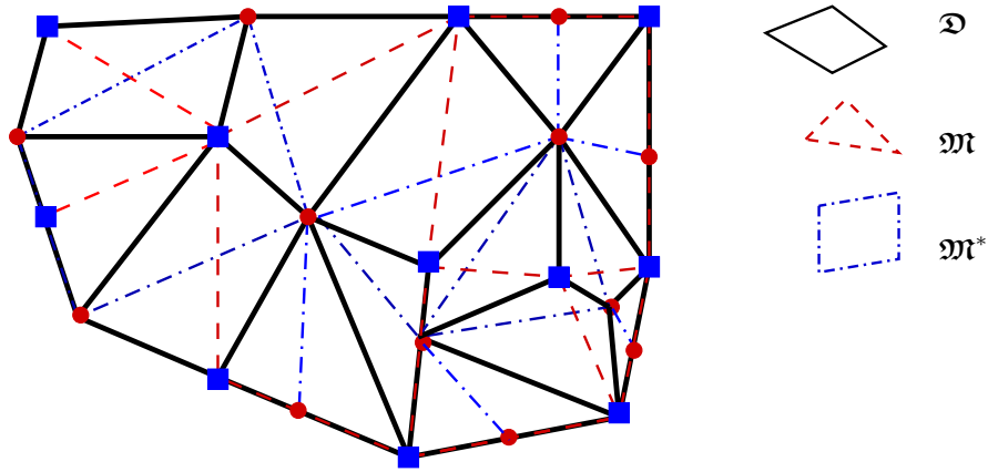
FIG. 9.1. Construction of \mathcal{T} from the diamond set \mathfrak{D}
