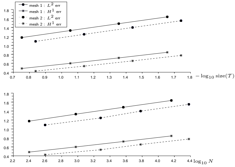
FIG. 8.2. Test case 1 : Anisotropic laplace equation (1.3) for the exact solution u_{0.5}^1
