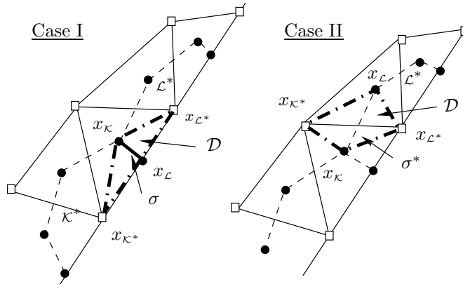
FIG. 3.1. Boundary dual control volumes and diamonds
