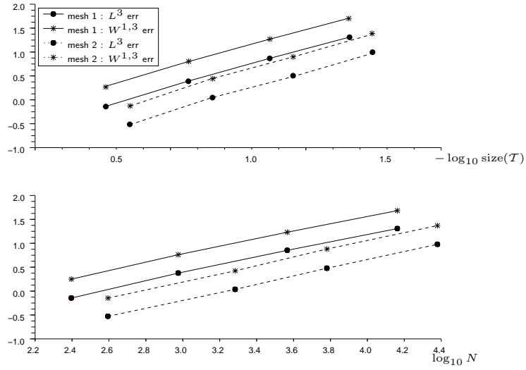
FIG. 8.4. Comparison between the meshes 1 and 2 for the p -laplacian (1.4) and the exact solution u_{0,2}^2
