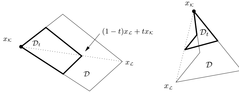
FIG. 7.1. The rescaled diamond D_t
