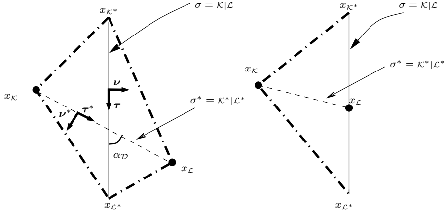
FIG. 2.2. Notations in a diamond cell \mathcal{D}_{\sigma, \sigma^*}
