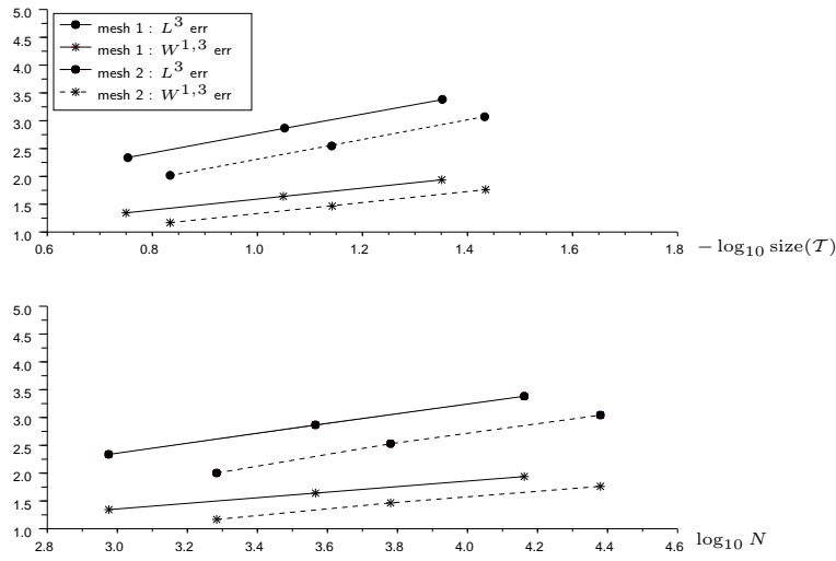
FIG. 8.3. Comparison between the meshes 1 and 2 for the model (1.5) and the exact solution u_{1.35}^1
