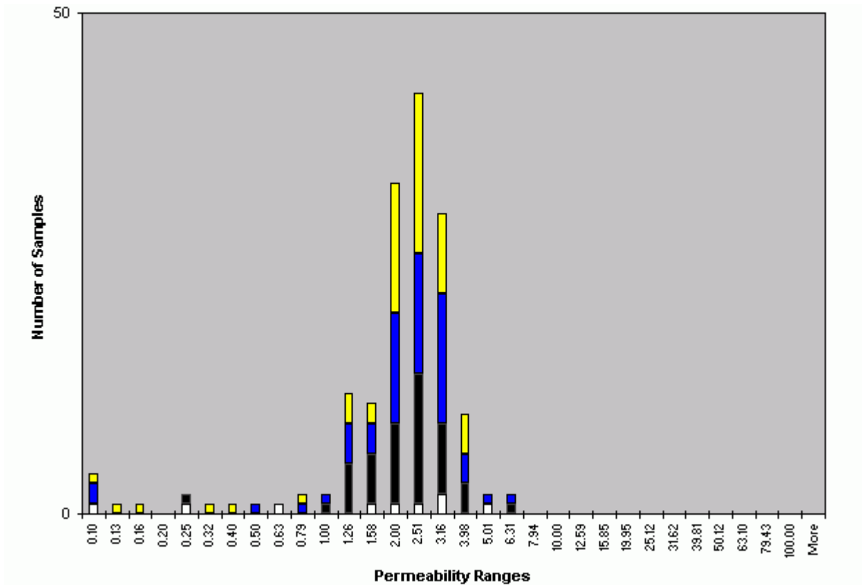
Figure 12: Permeability histogram for RR-0.45 ("E") in layer 10 (all wells).
