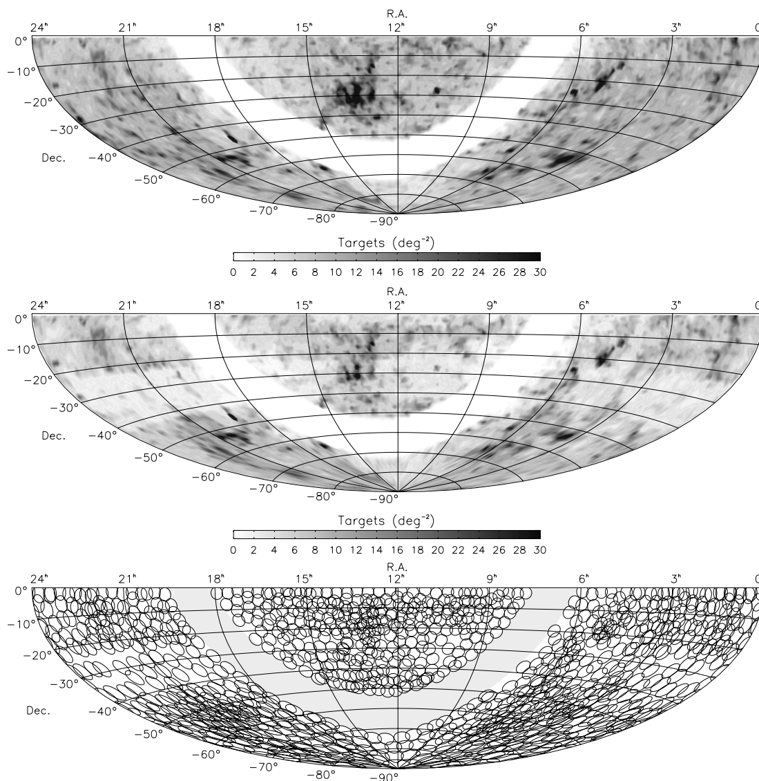
Figure 3. (Top) Sky distribution of all targets in the source catalogues. (Middle) Distribution of unobserved sources at the time of the version D tiling allocation in 2003 February. Note how most of the fields observed between the versions A and D were confined to the central strip ( -23^\circ to -42^\circ declination). (Bottom) Optimal distribution of tiles based on the unobserved sources at the time of version D.
