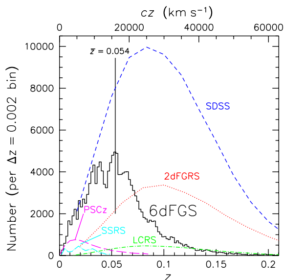
Figure 10. A colour version of this figure appears in the online version of the journal. Number–redshift distribution for the 6dF Galaxy Survey, comprising First Data Release galaxies with redshift quality Q \geq 3 and cz > 600 \text{ km s}^{-1} . The mean redshift for the survey ( \bar{z} = 0.054 ) is indicated with a vertical solid line. Also shown are the equivalent distributions for the SDSS (short dashed line, blue), 2dFGRS (dotted line, red), PSCz (long dashed line, magenta), SSRS (dot-dash line, cyan) and LCRS (dot-dash line, green) surveys listed in Table 1. All curves have been normalized to yield the total sample sizes given in Table 1.
