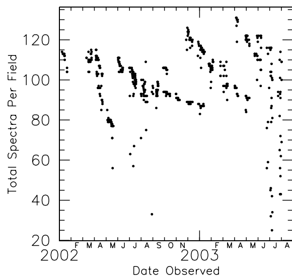
Figure 2. Total number of spectra obtained per field between 2002 January and 2003 June. The upper envelope shows the maximum number of fibres available at any one time. It tracks the loss of fibres over time, and how field plate #1 was taken out of service for 2003 January–February for a major fibre repair. The large scatter seen from the end of 2003 June is due to a change in observing strategy, from field choice maximizing fibre allocation to one aimed at completing areas of sky.
