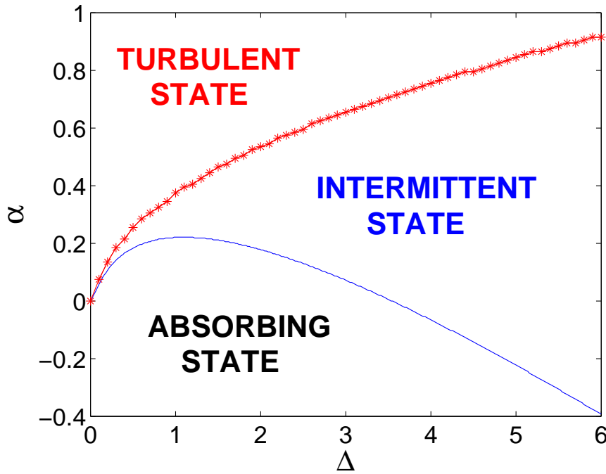
Fig. 5. Bifurcation diagram of the noisy oscillator (2) for \beta = 3 . The straight line curve correspond to the condition (15) and the one with “+” sign to the condition (16).
