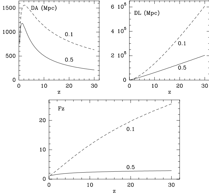
Fig. 3. Angular size distance ( D_A ), luminosity distance ( D_L ) and correction factor F_z = \left(\frac{D_L H_0}{cz}\right)^2 , for two values of q_0 (0.5 full line, 0.1 dashed line).
