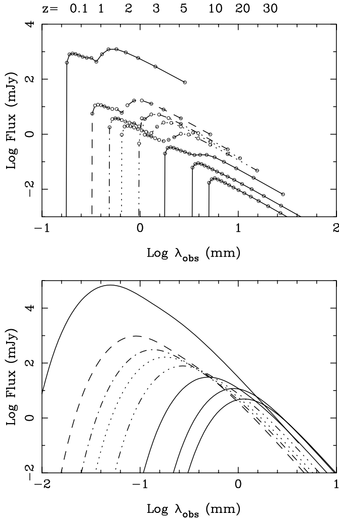
Fig. 4. Expected flux for the two-component cloud model, for various redshifts z = 0.1, 1, 2, 3, 5, 10, 20, 30 , and q_0 = 0.5 . Top are the CO lines, materialised each by a circle. Bottom is the continuum emission from dust. It has been assumed here that T_{dust}^6 - T_{bg}^6 is conserved.
