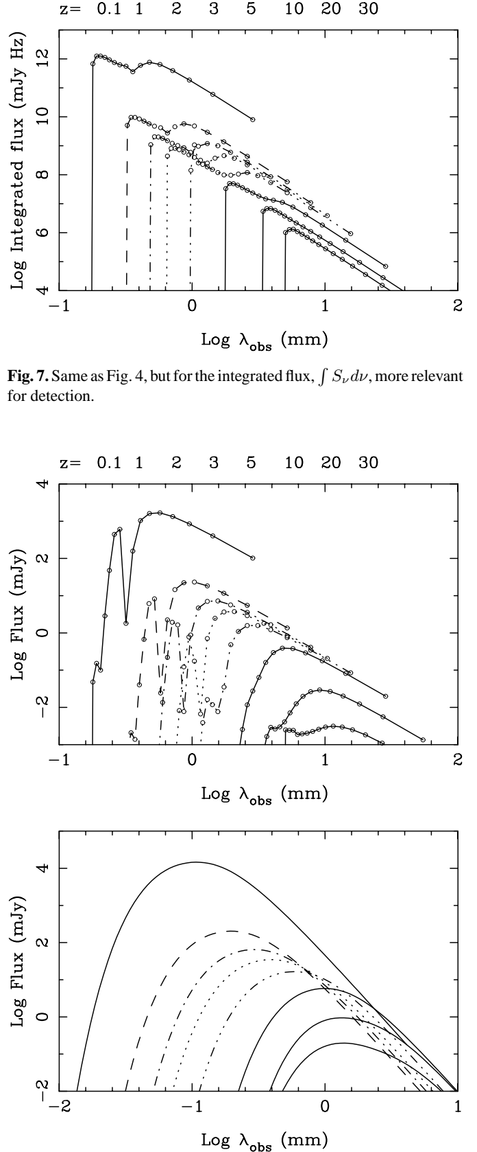
Fig. 8. Same as Fig. 4, but with the homogeneous sphere model, with T_d = 50 K. The non monotonous behaviour is due to excitation far from LTE (see Sect. 2.2)
