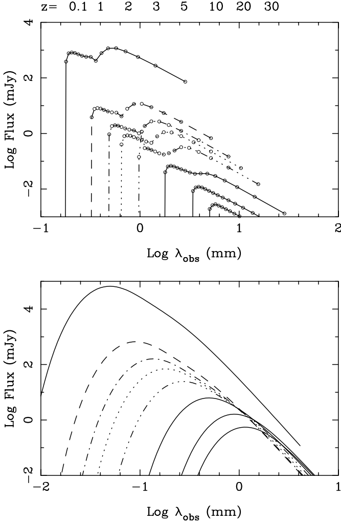
Fig. 6. Same as Fig. 4, but with q_0 = 0.1 .
