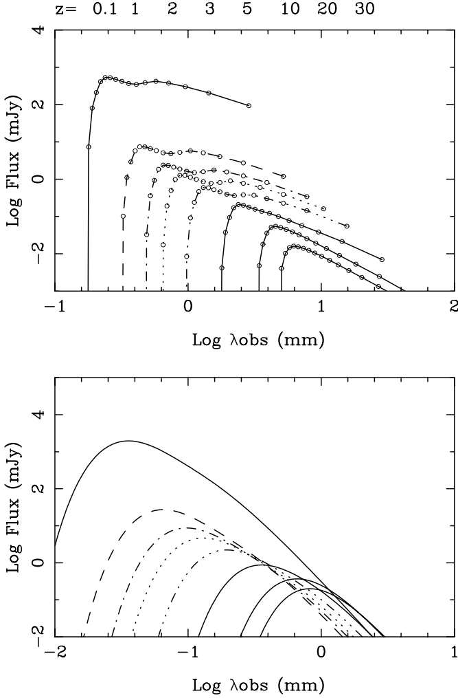
Fig. 10. Same as Fig. 4, but for one optically thin model, with \text{CO}/\text{H}_2 = 10^{-6} .
