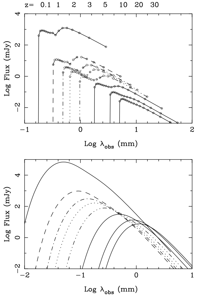
Fig. 5. Same as Fig. 4, but with T_{dust}^4 - T_{bg}^4 conserved, as for an optically thick medium (see text for details).
