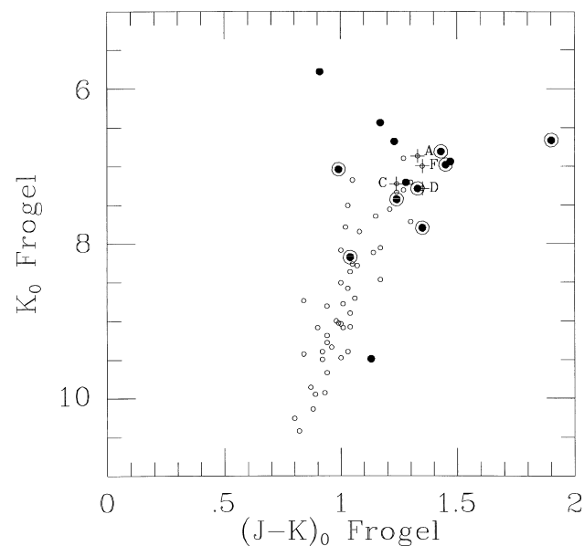
Figure 7. (J - K)_0 , K_0 diagram for ISOGAL objects in the NGC 6522 field that have photometry by Frogel & Whitford (1987) or Tiede et al. (1995) on the CIT/CTIO system. The NGC 6522 Miras are indicated by heavy points. Other high mass-loss objects specially examined (see below, Section 6) are crossed. Also shown as circled points are Miras in our Sgr I field, taken from Glass et al. (1995). The tip of the RGB is estimated to occur at K \sim 8.2 . Note that the NGC 6522 Mira brightest at K (= TLED9) appears unusually blue in the Frogel & Whitford photometry. It was considerably redder when measured by Glass & Feast (1982).
