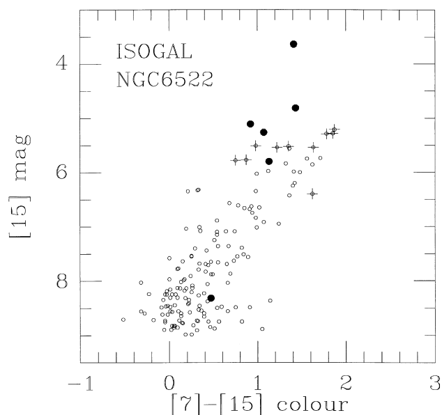
Figure 8. ISOCAM colour–magnitude diagram for the 15 \times 15 arcmin 2 field in the NGC 6522 Window. Note that many sources are detected only at 7 \mu\text{m} and do not appear here. Known Mira variable stars are indicated by heavy points and some other stars chosen for investigation as possible high mass-loss objects are crossed. The [7]-[15] colours make use only of the second LW2 exposure, which was nearly simultaneous with the LW3.
