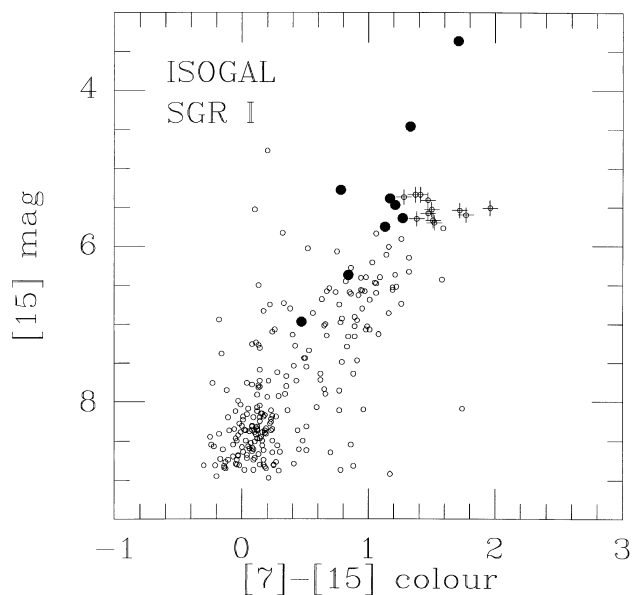
Figure 9. ISOCAM colour–magnitude diagram for the 15 \times 15 arcmin 2 field in the Sgr I Window. See caption of Fig. 8 for further details.
