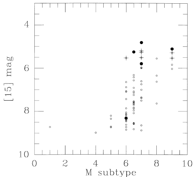
Figure 12. 15- \mu\text{m} mag versus M subtype for a subset of stars in the NGC 6522 field with 15- \mu\text{m} detections and spectroscopic information available. Symbols as in previous figure.
