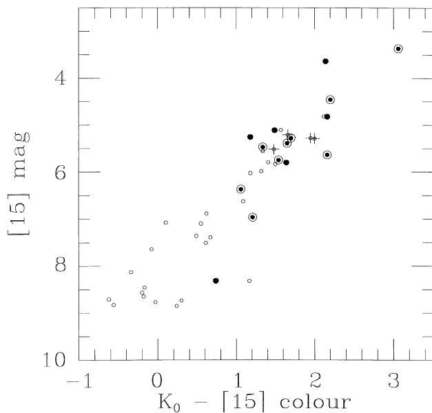
Figure 11. 15- \mu\text{m} mag versus K_0 -[15] for a subset of stars in the NGC 6522 field detected at 15 \mu\text{m} and observed (not simultaneously) at K by Frogel & Whitford (1987). Mira variables are indicated by heavy points. Other high mass-loss stars are crossed (see below). For convenience, the Miras in Sgr I (with K photometry from Glass et al. 1995) are also plotted (circled points).
