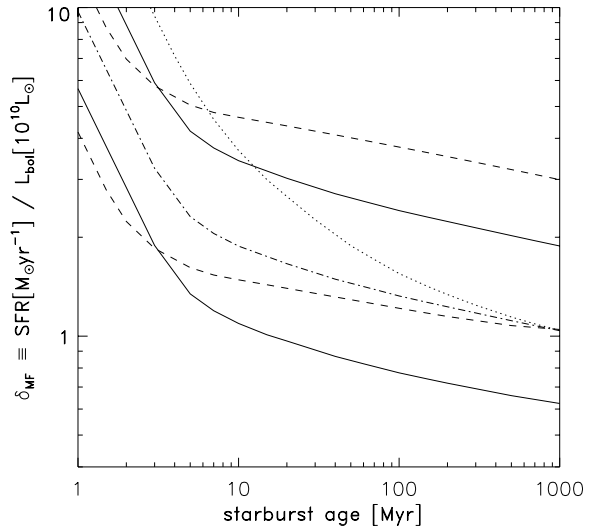
Fig. 3. Star formation rate per total luminosity, \delta_{\text{MF}} , for continuous starbursts as a function of starburst age, adopting different IMFs. Solid lines: Salpeter IMF with m_1 = 0.1 M_\odot (upper solid line) and m_1 = 1.6 M_\odot (lower solid line), with stellar lifetimes and luminosities taken from Schaerer et al. (1993) evolution tracks. Dashed lines: as for solid lines, but adopting approximate lifetimes and luminosities from Telesco & Gatley (1984). Dash-dotted line: like upper solid line but assuming a flat IMF below 1 M_\odot . Dotted line: as upper solid line, but assuming a log-normal IMF: d \log N/d \log m = -\log m .
