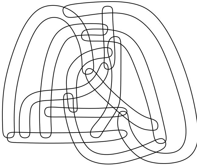
Figure 6: A planar circle diagram for the icosahedral graph \Delta_\Gamma .
