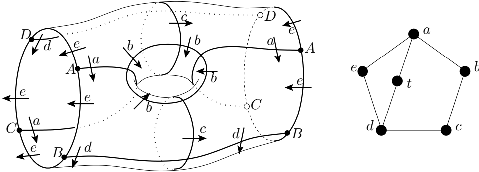
Figure 5: We obtain the surface F by identifying the two boundary circles of the surface on the left. The fundamental group of the complex X embeds in G(\Delta) , where \Delta is the graph on the right.
