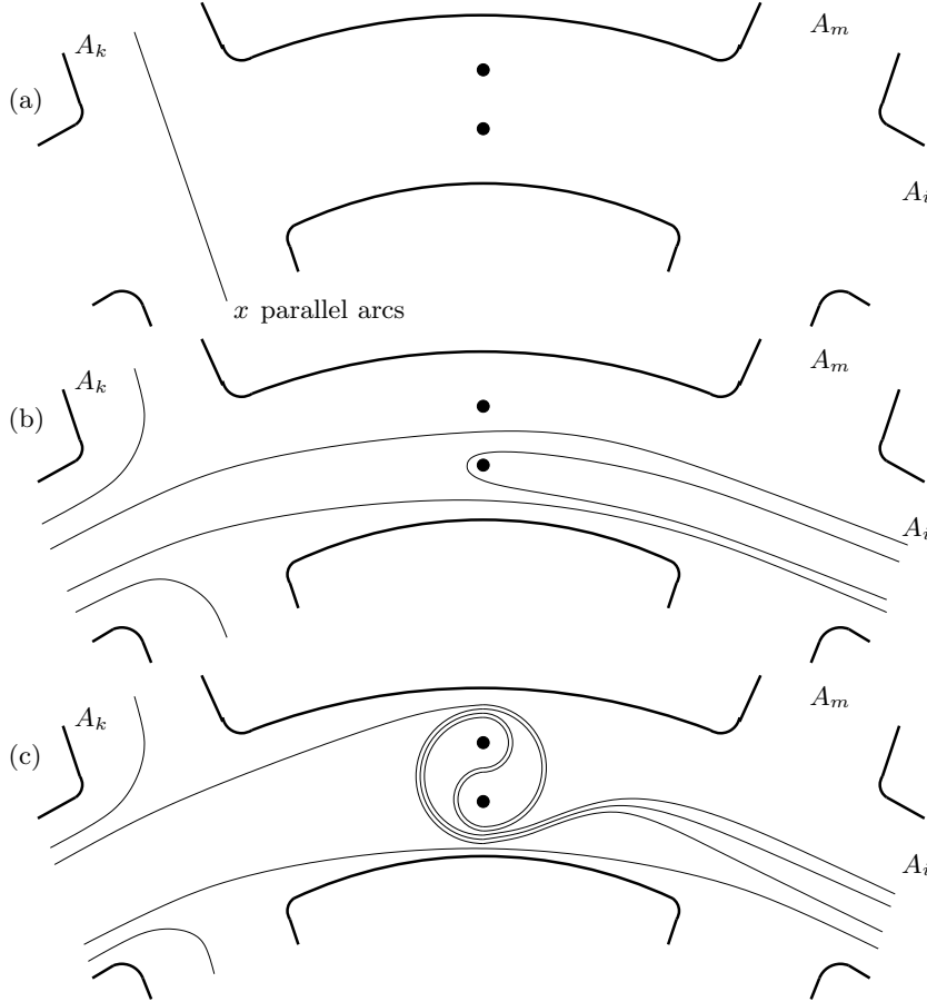
Figure 3: If there are x arcs traversing a square of A_i \cap A_k in the A_k -direction, then after the action of \widehat{f}(a_i) there are 2x arcs traversing any square of intersection involving A_i in the A_i -direction. (Part (b) shows the result of the action by \tau_{B_i} \circ \tau_{D_i}^2 \circ \tau_{C_i}^{-2} .)
