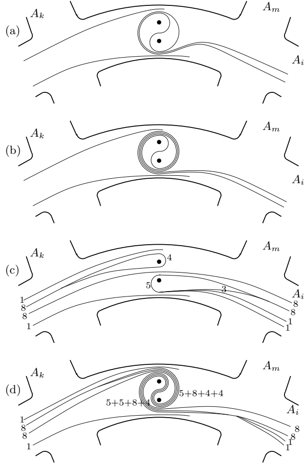
Figure 4: Acting by \widehat{f}(a_i) twice in a row. (a) After the first action by \widehat{f}(a_i) . (b) After the action by \tau_{B_i} . (c) After the action by \tau_{C_i}^2 \tau_{D_i}^{-2} . (d) After the action by \tau_{B_i} .
