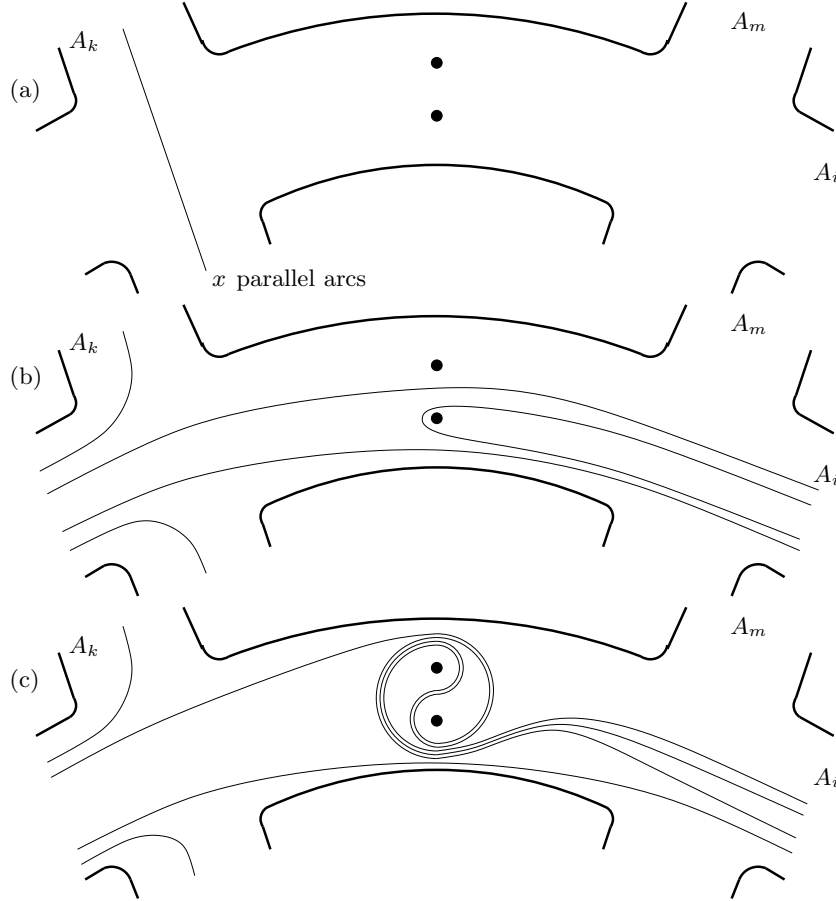
Figure 3: If there are x arcs traversing a square of A_i \cap A_k in the A_k -direction, then after the action of \widehat{f}(a_i) there are 2x arcs traversing any square of intersection involving A_i in the A_i -direction. (Part (b) shows the result of the action by \tau_{B_i} \circ \tau_{D_i}^2 \circ \tau_{C_i}^{-2} .)
